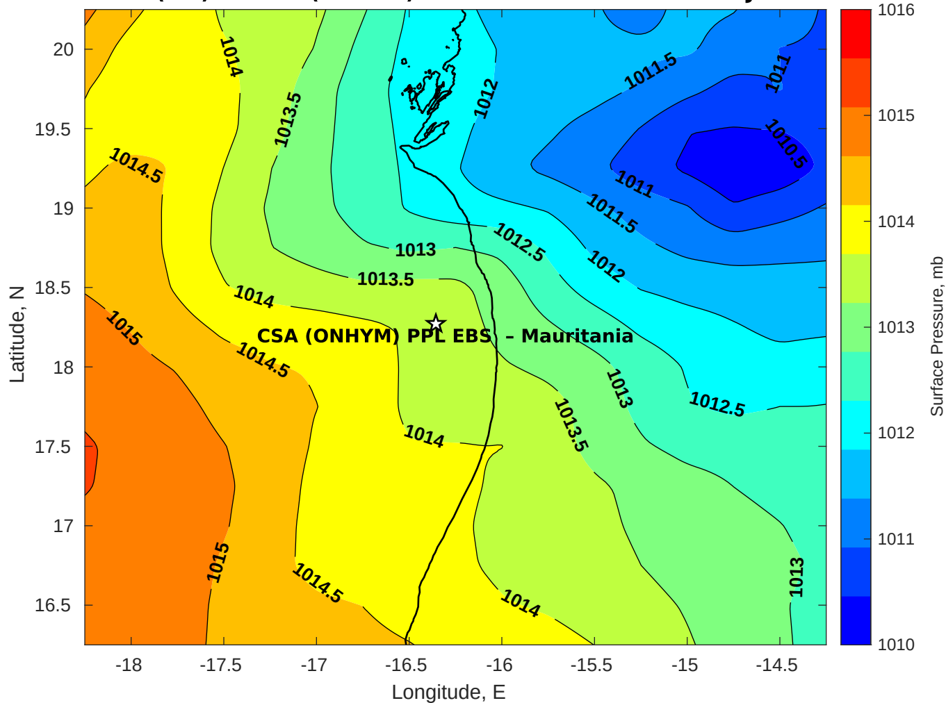
Surface Pressure (mb) for CSA (ONHYM) PPL EBS - Mauritania at 17-Jun-2025 00:00:00
