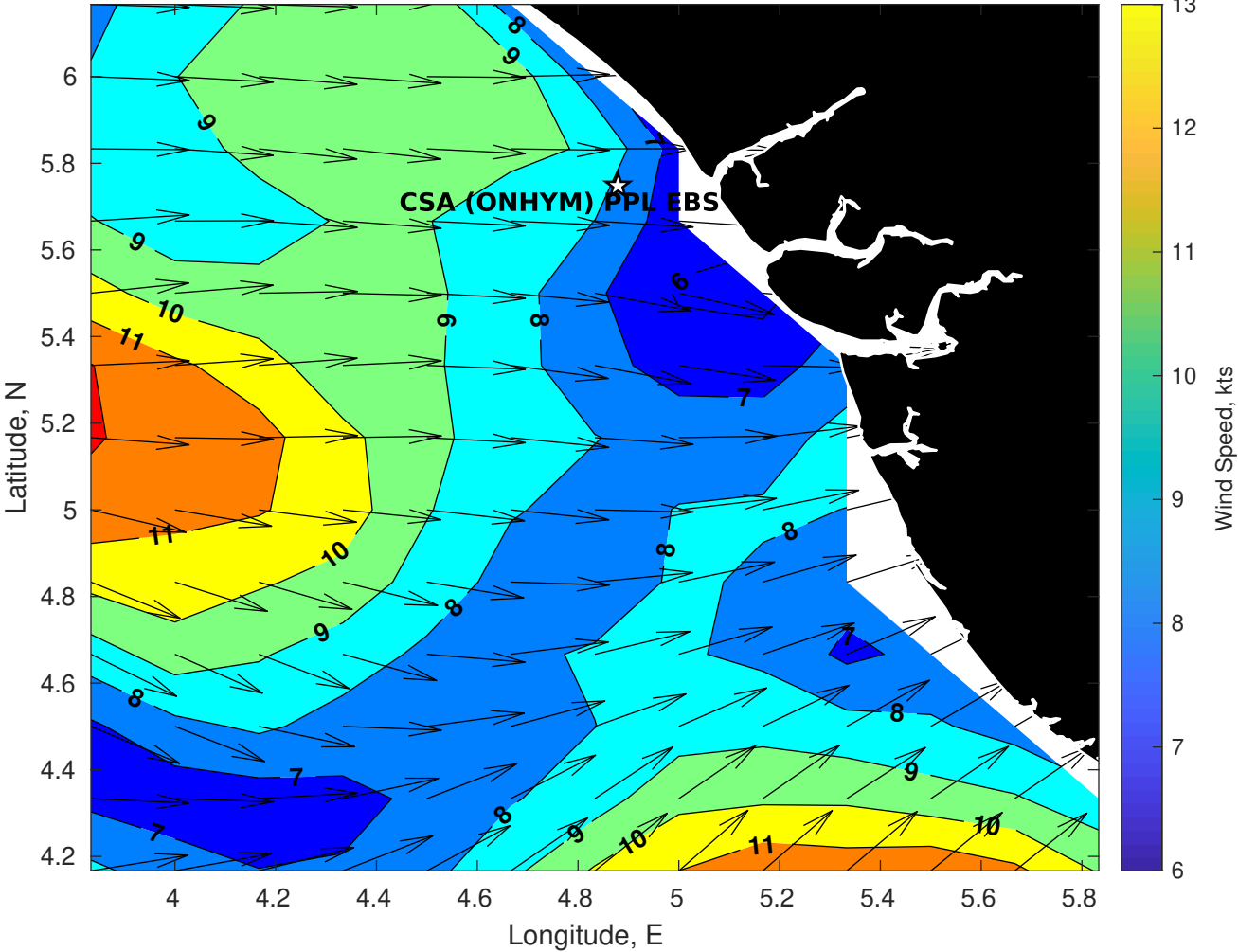
Winds (kts) for CSA (ONHYM) PPL EBS - Nigeria at 15-Jun-2025 09:00:00
