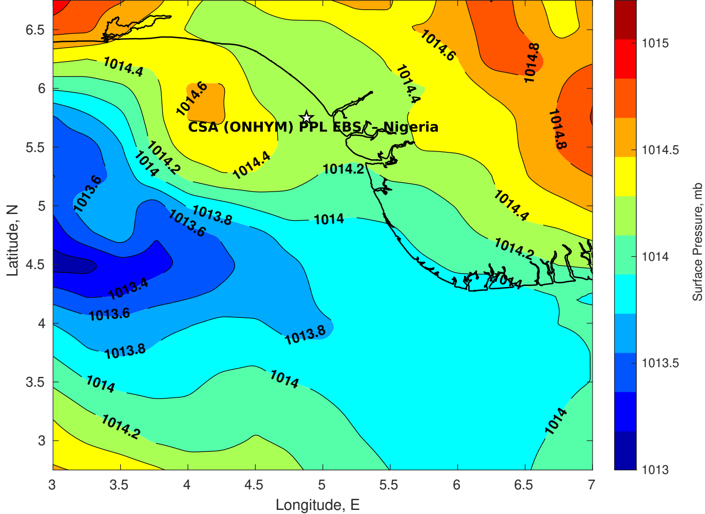
Surface Pressure (mb) for CSA (ONHYM) PPL EBS - Nigeria at 15-Jun-2025 00:00:00
