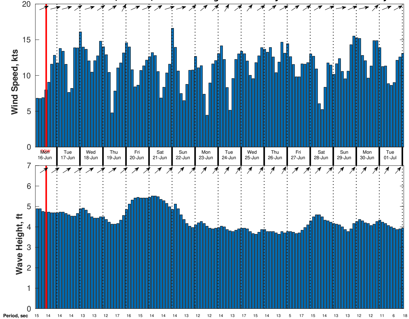
Wind & Wave Forecast for CSA (ONHYM) PPL EBS - Nigeria from 15-Jun-2025 02:00:00 to 01-Jul-2025 02:00:00
