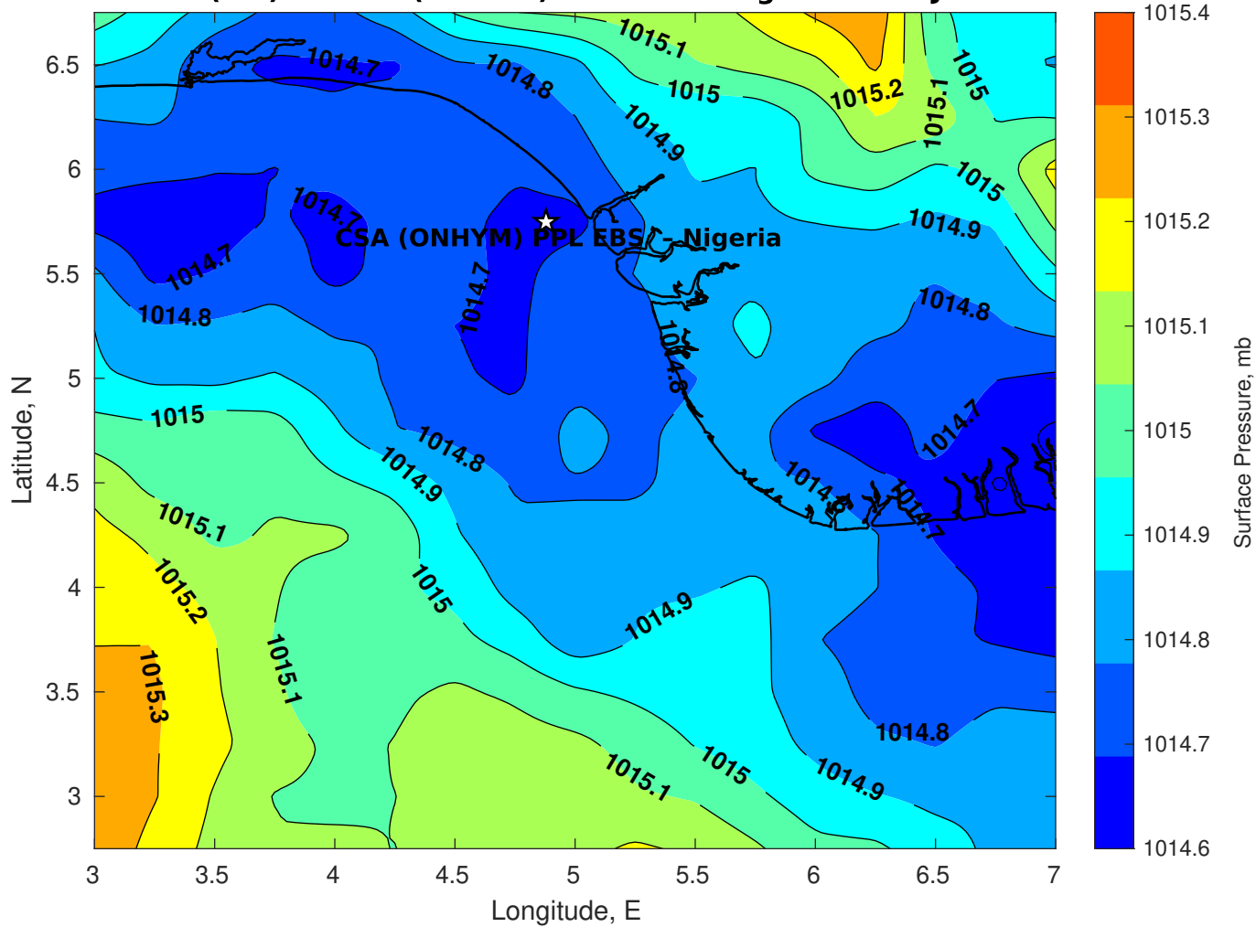
Surface Pressure (mb) for CSA (ONHYM) PPL EBS - Nigeria at 16-Jun-2025 00:00:00
