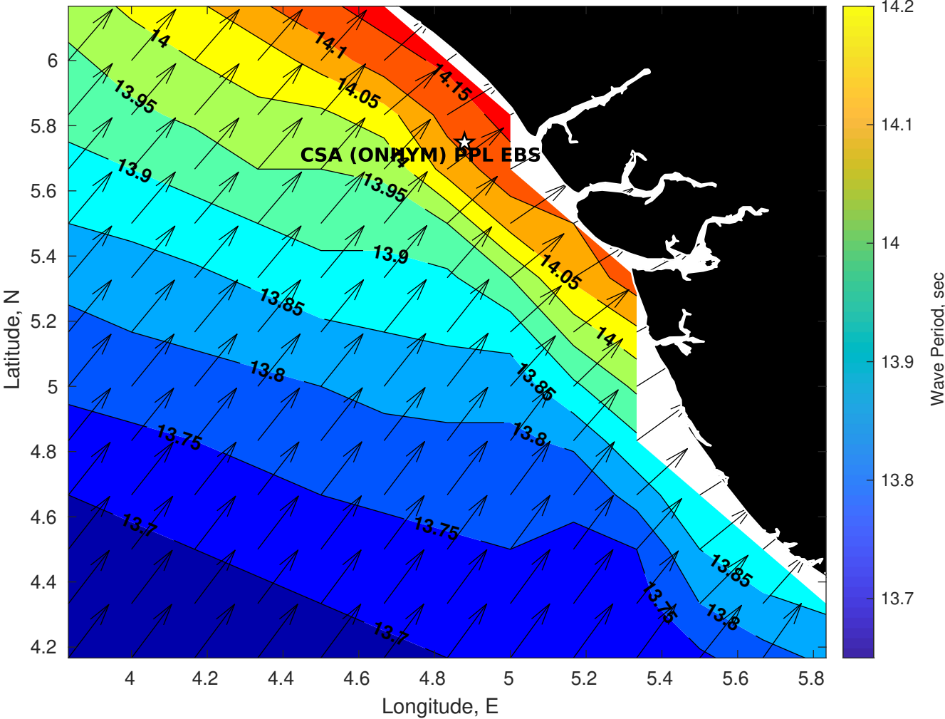
Wave Period (sec) for CSA (ONHYM) PPL EBS - Nigeria at 15-Jun-2025 09:00:00
