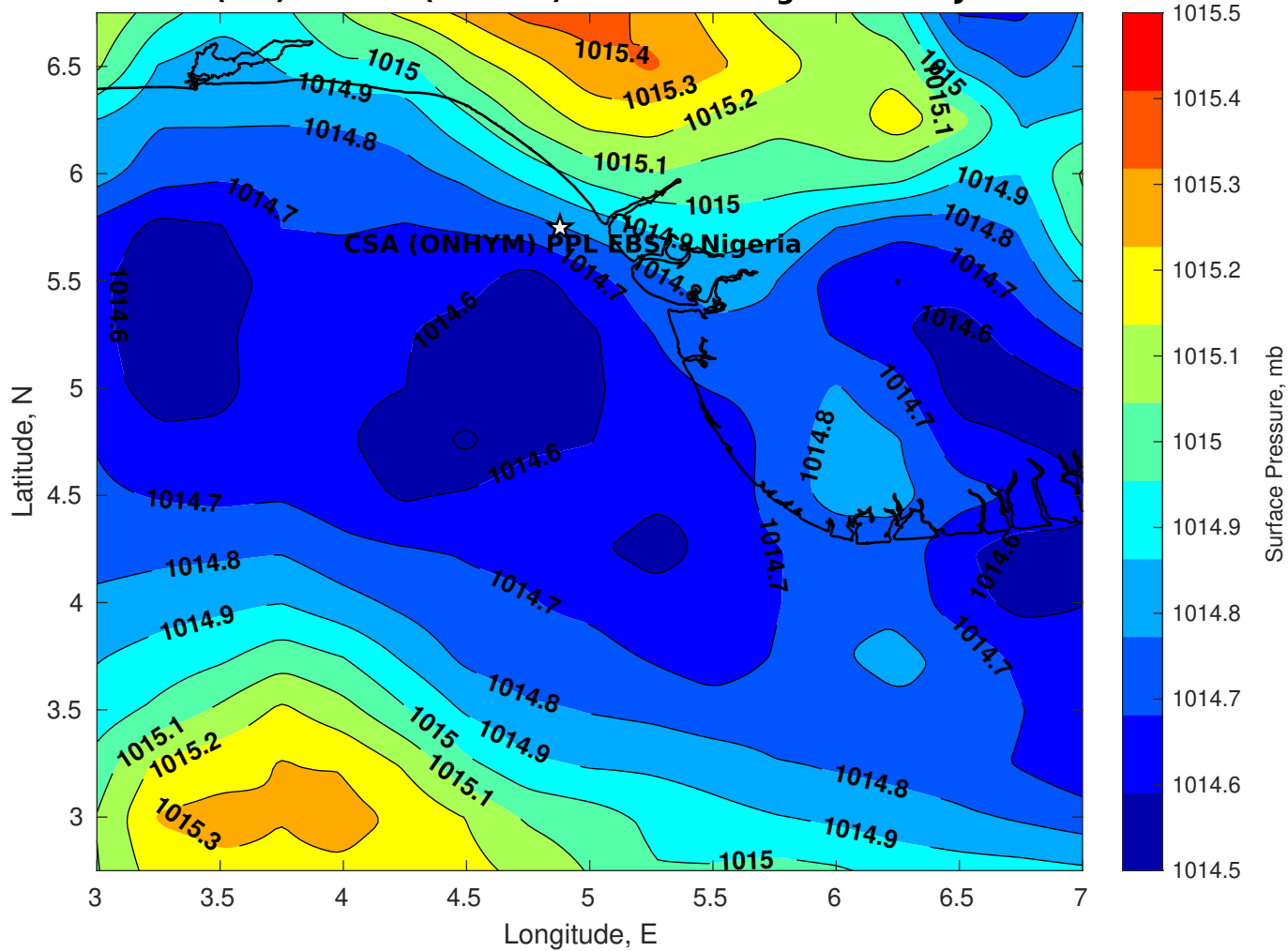
Surface Pressure (mb) for CSA (ONHYM) PPL EBS - Nigeria at 17-Jun-2025 00:00:00
