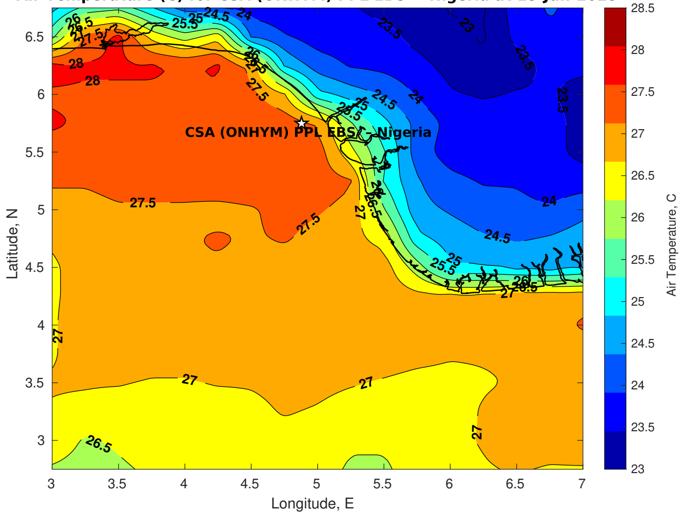
Air Temperature (C) for CSA (ONHYM) PPL EBS - Nigeria at 15-Jun-2025
