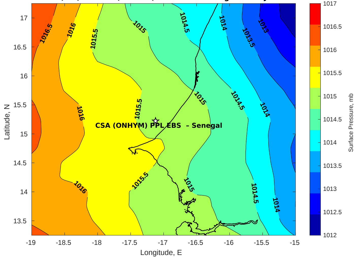
Surface Pressure (mb) for CSA (ONHYM) PPL EBS - Senegal at 15-Jun-2025 00:00:00
