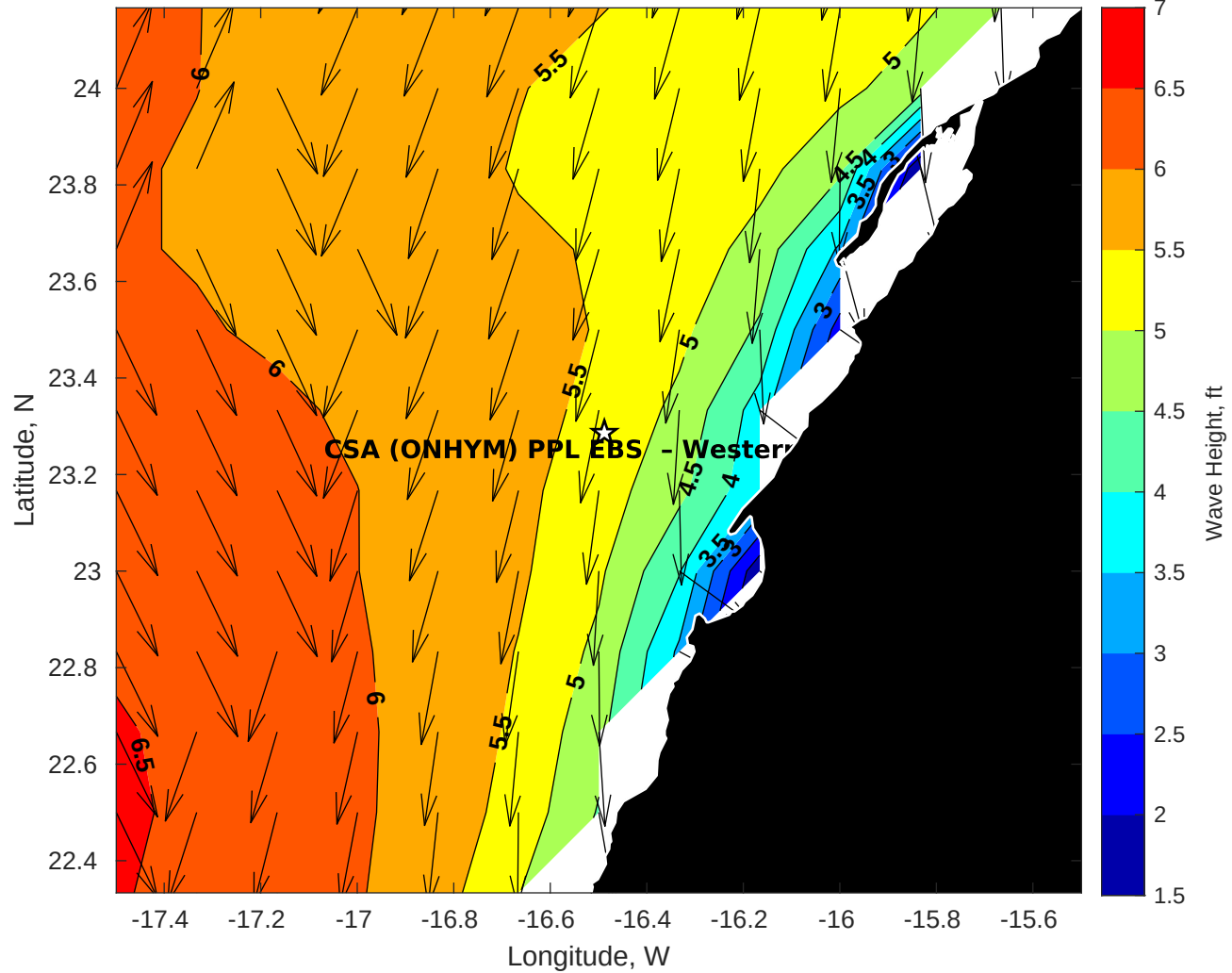
Wave Height (ft) for CSA (ONHYM) PPL EBS - Western Sahara at 15-Jun-2025 09:00:00
