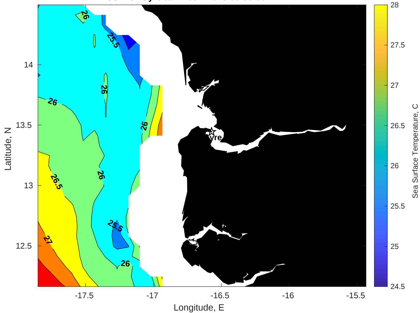
SST for Gyre at 17-Jun-2025 00:00:00
