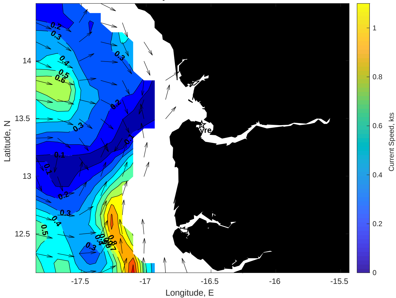
Surface Currents for Gyre at 17-Jun-2025 00:00:00
