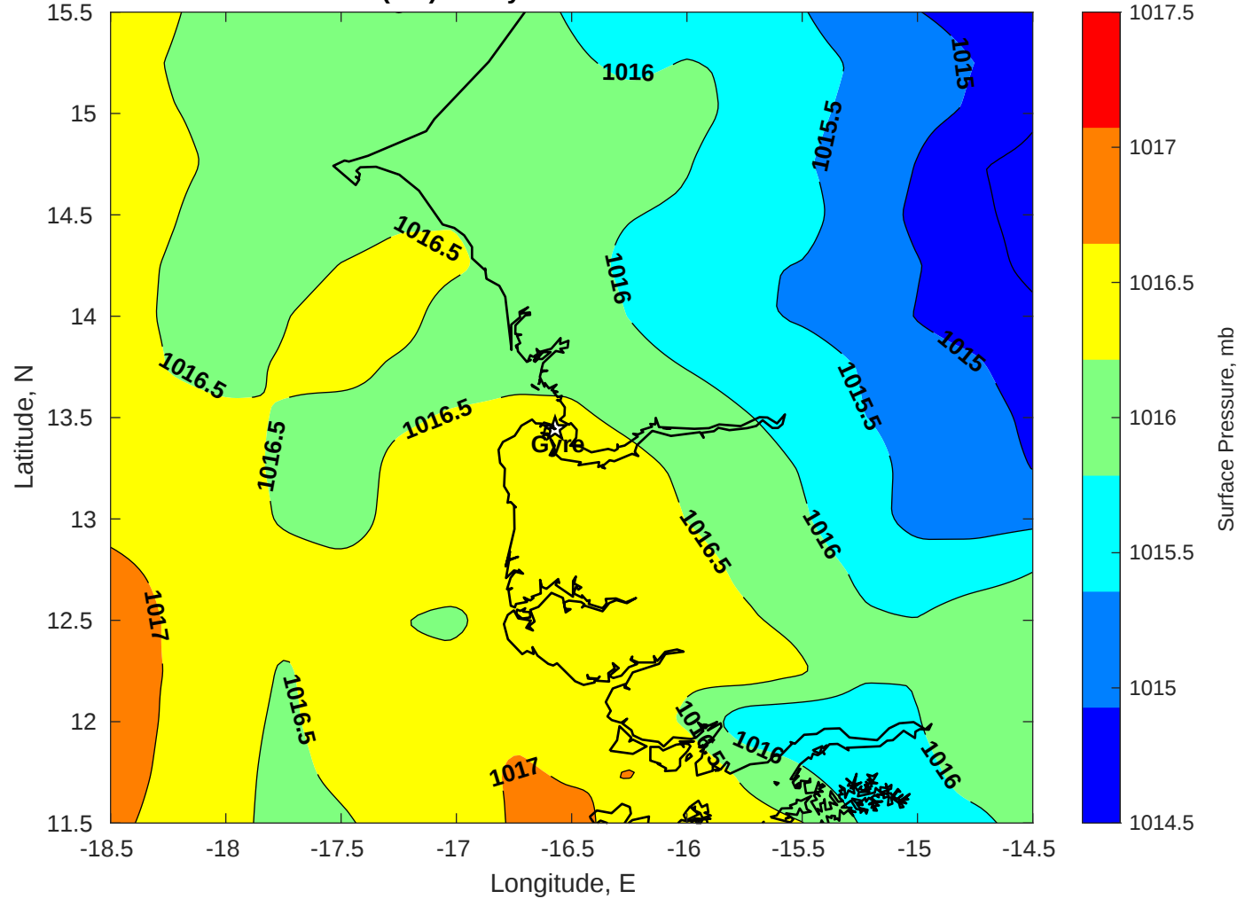
Surface Pressure (mb) for Gyre at 18-Jun-2025 00:00:00
