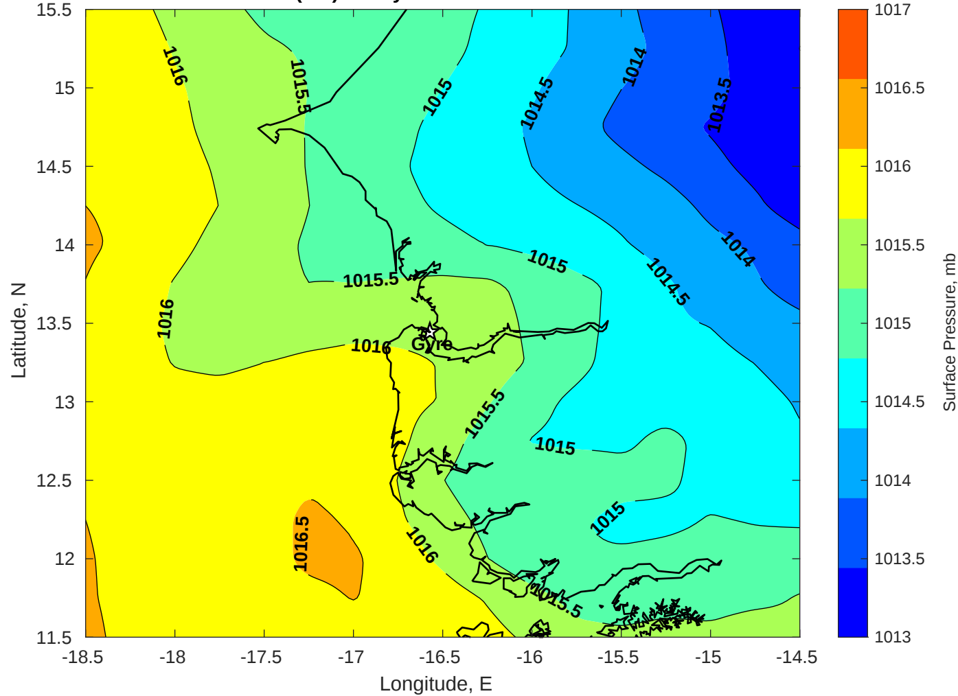
Surface Pressure (mb) for Gyre at 19-Jun-2025 00:00:00
