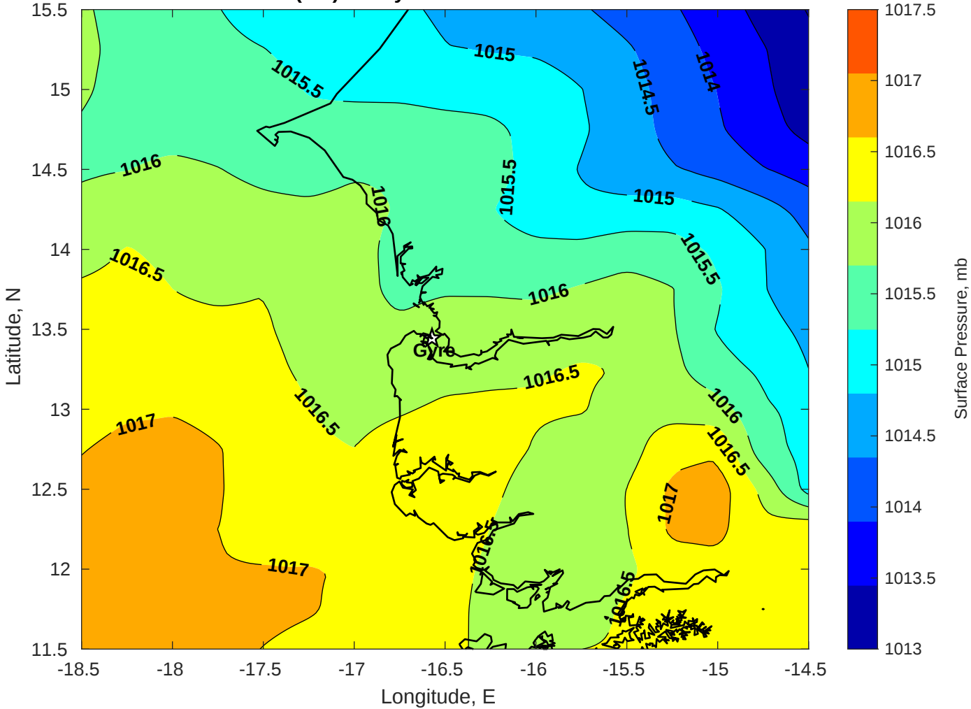
Surface Pressure (mb) for Gyre at 20-Jun-2025 00:00:00
