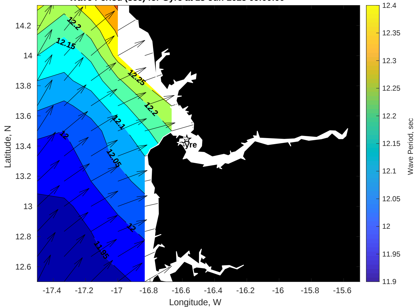
Wave Period (sec) for Gyre at 18-Jun-2025 09:00:00
