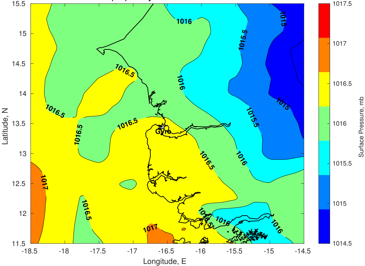
Surface Pressure (mb) for Gyre at 18-Jun-2025 00:00:00
