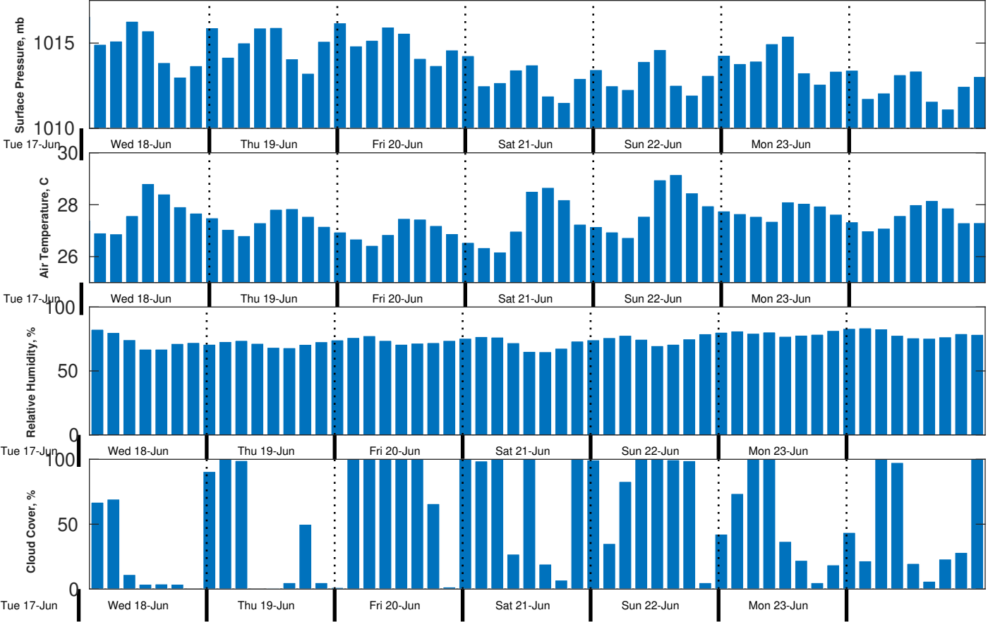
Met Forecast for Gyre from 17-Jun-2025 23:00:00 to 24-Jun-2025 23:00:00
