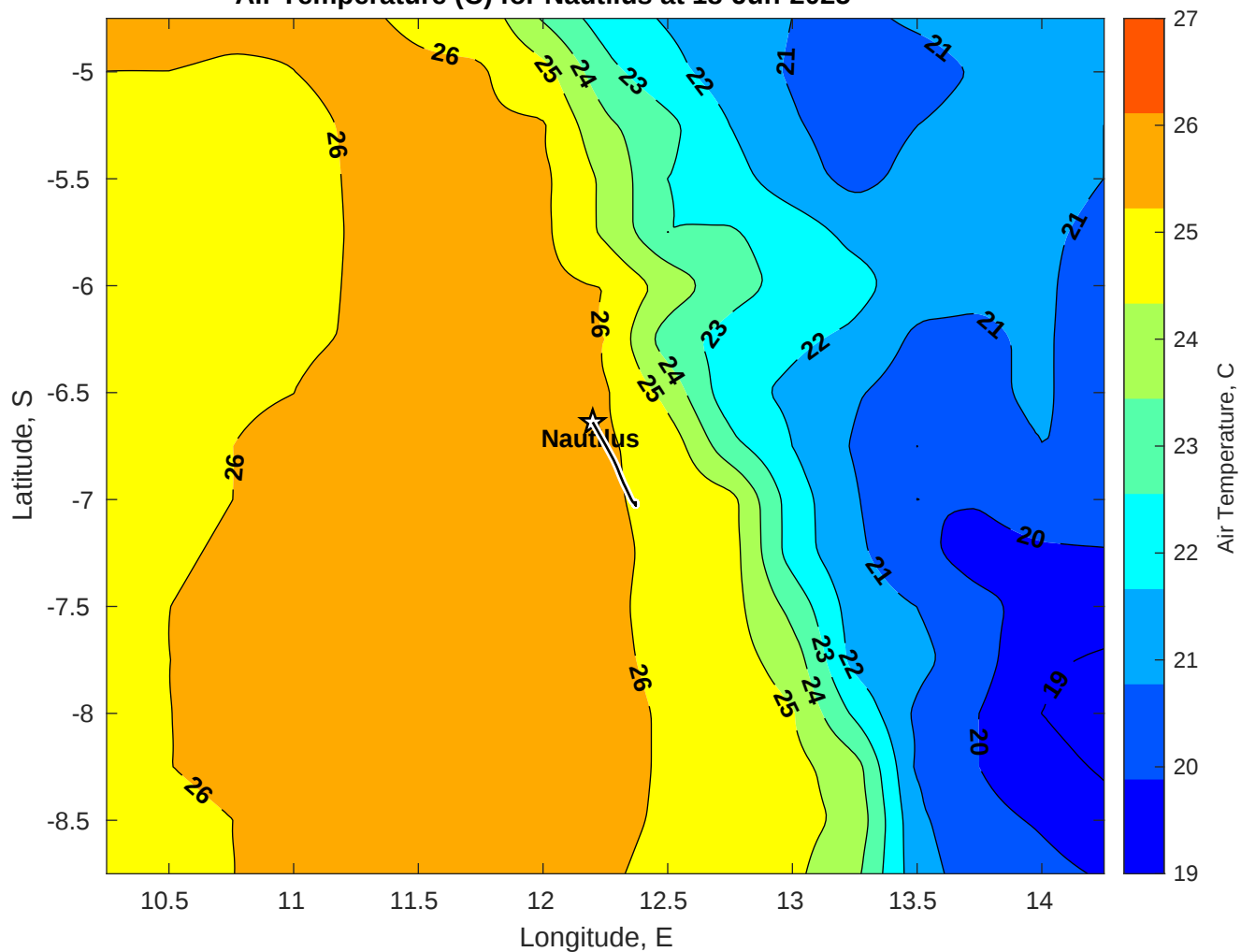
Air Temperature (C) for Nautilus at 18-Jun-2025
