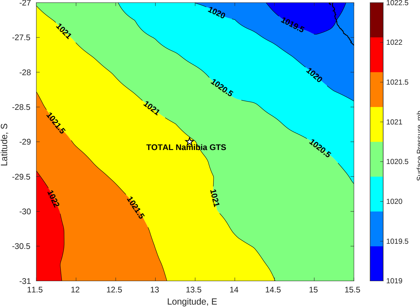
Surface Pressure (mb) for TOTAL Namibia GTS at 16-Jun-2025 00:00:00
