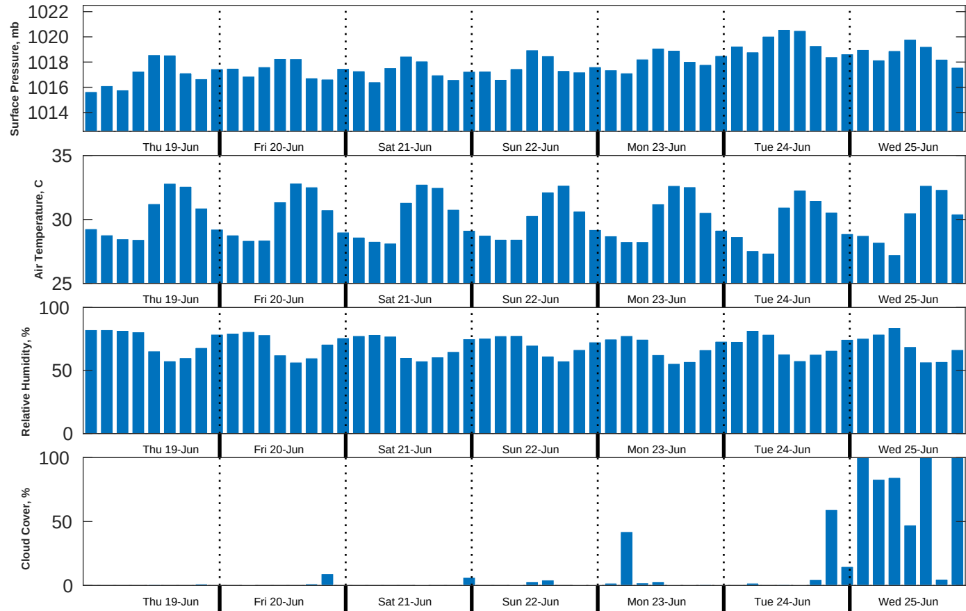
Met Forecast for Brooks McCall from 19-Jun-2025 00:00:00 to 26-Jun-2025 00:00:00
