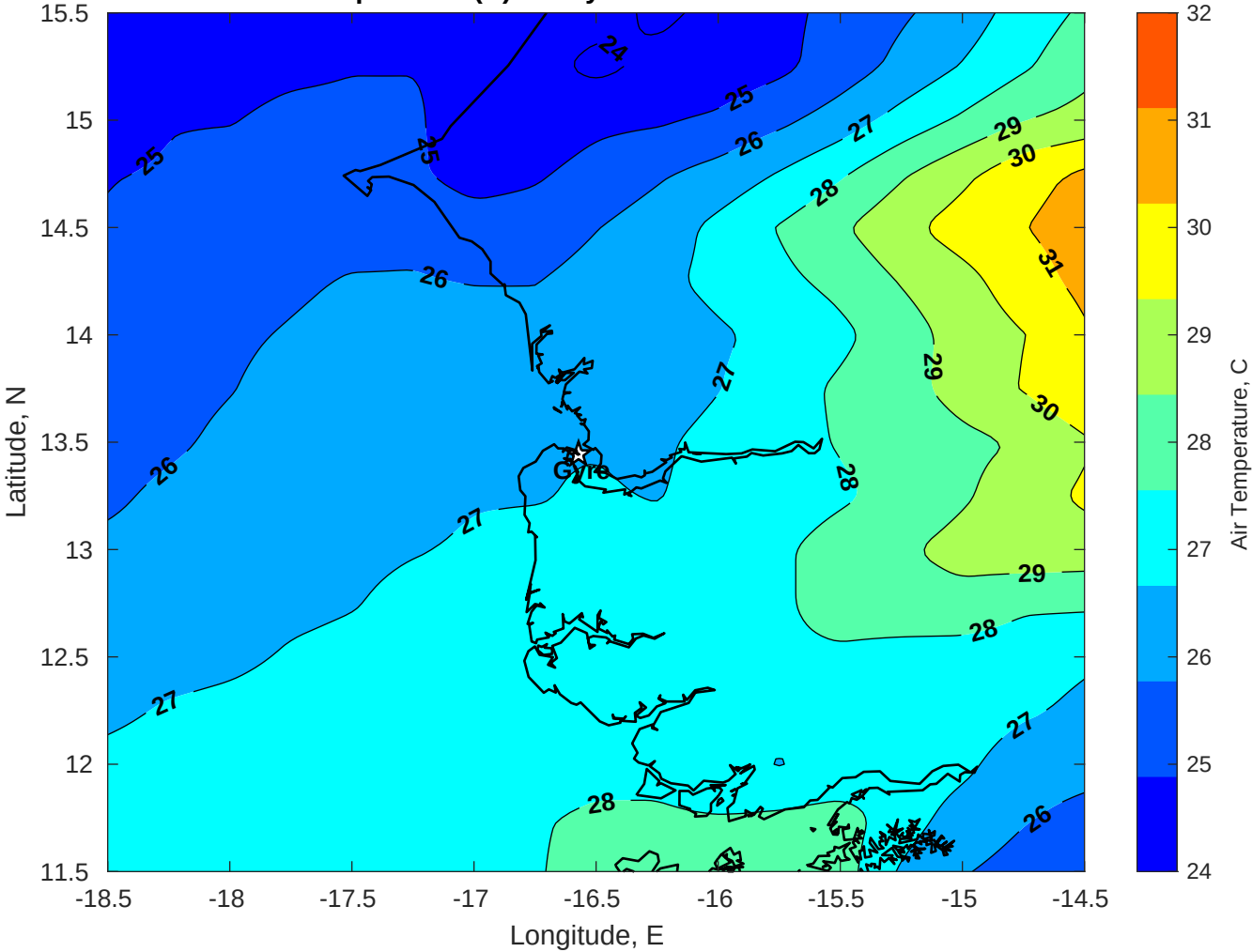
Air Temperature (C) for Gyre at 19-Jun-2025
