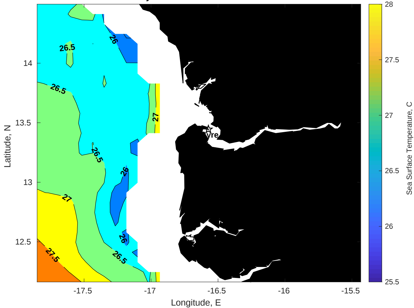
SST for Gyre at 18-Jun-2025 00:00:00
