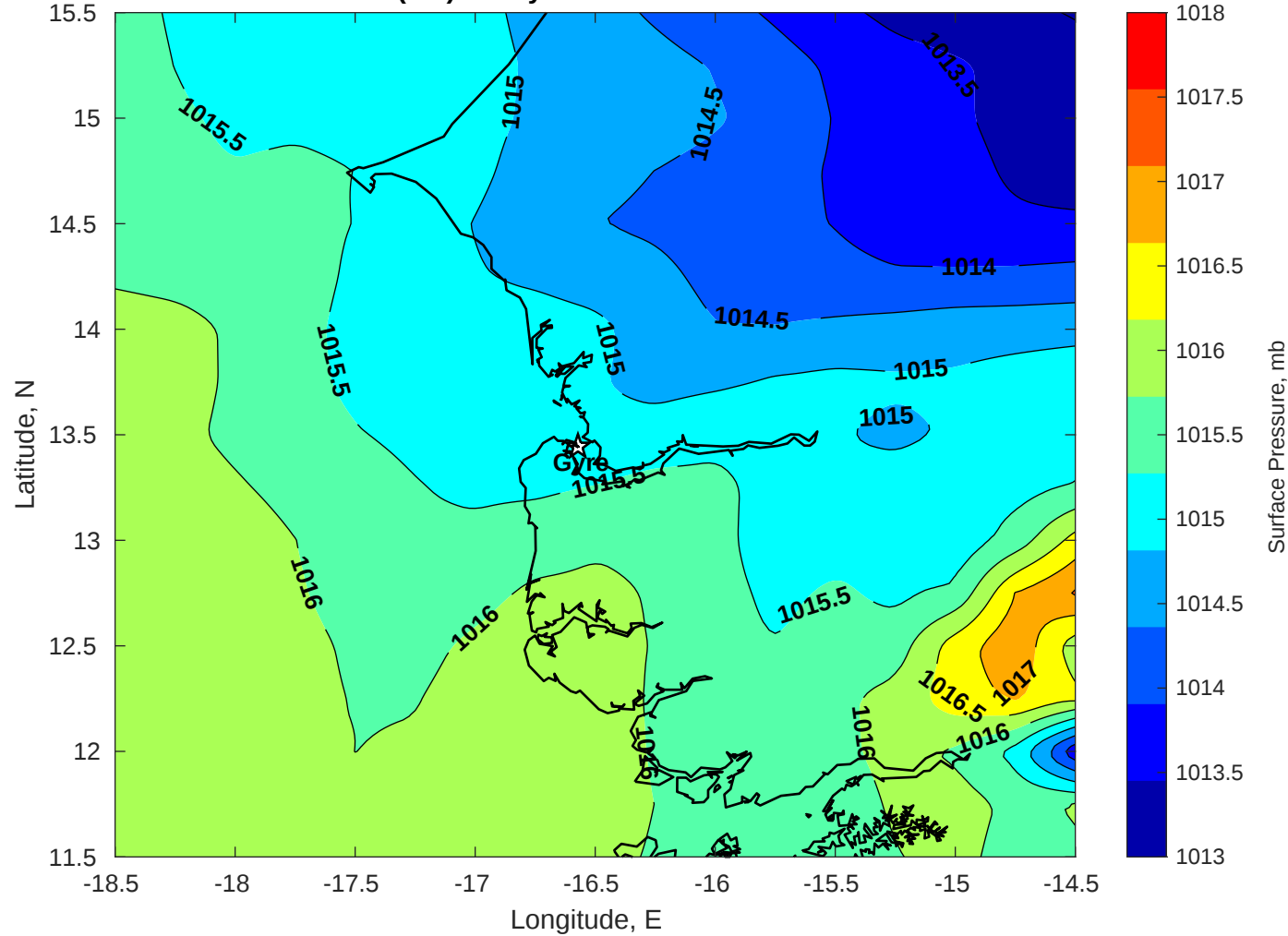
Surface Pressure (mb) for Gyre at 20-Jun-2025 00:00:00
