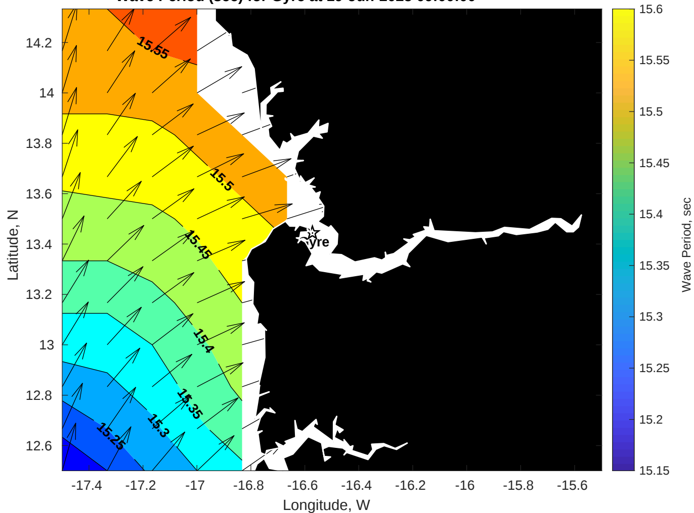
Wave Period (sec) for Gyre at 19-Jun-2025 09:00:00
