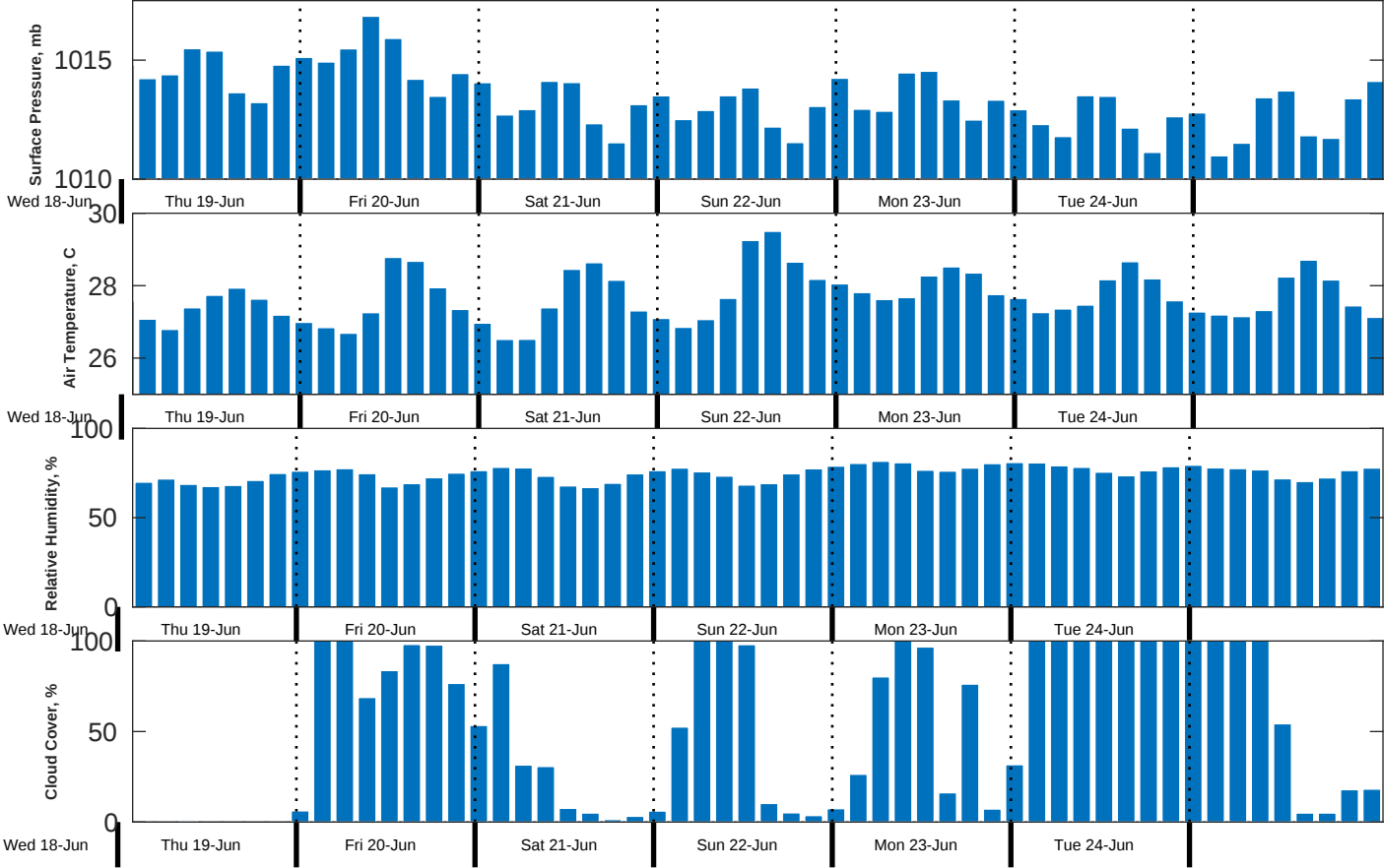
Met Forecast for Gyre from 18-Jun-2025 23:00:00 to 25-Jun-2025 23:00:00
