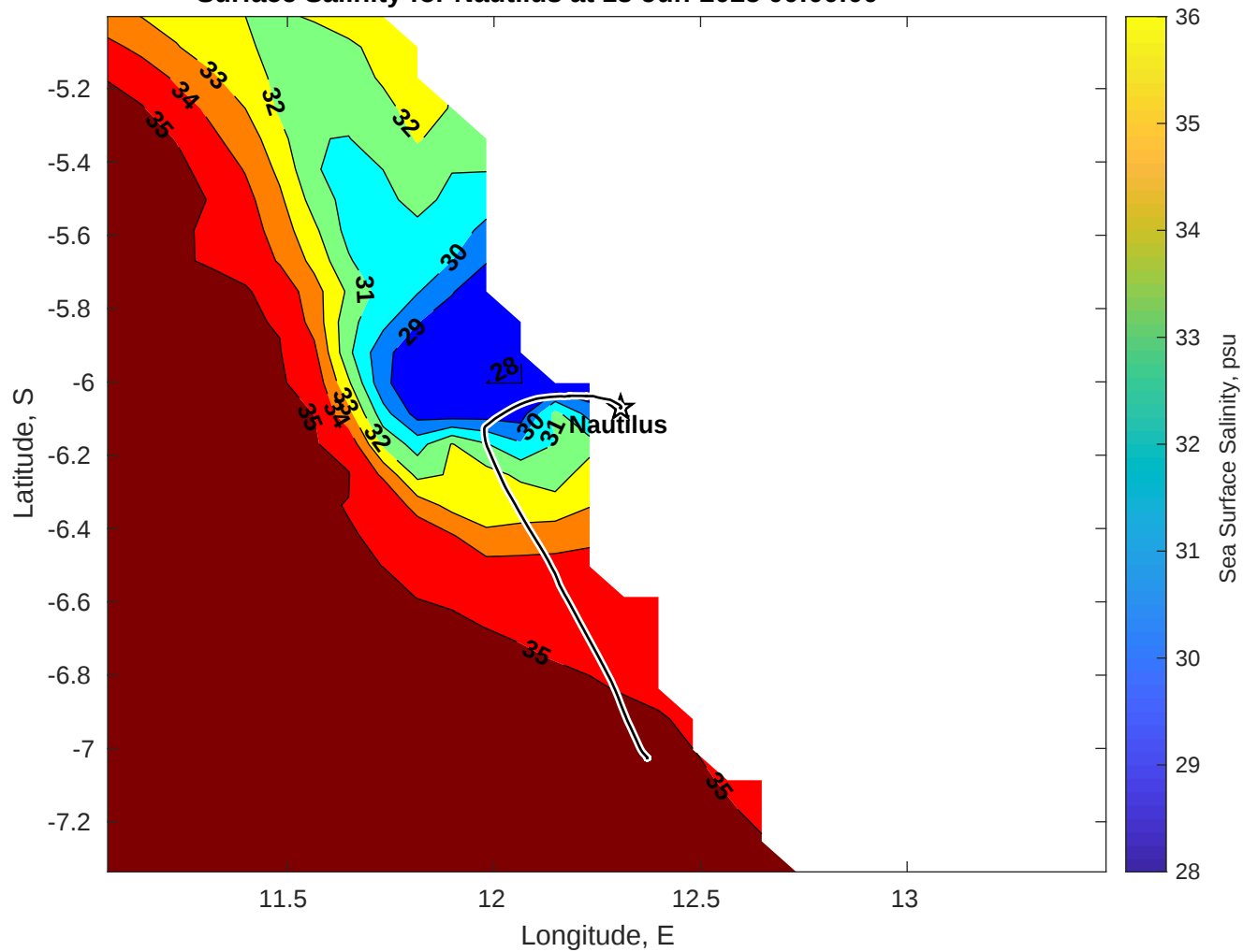
Surface Salinity for Nautilus at 18-Jun-2025 00:00:00
