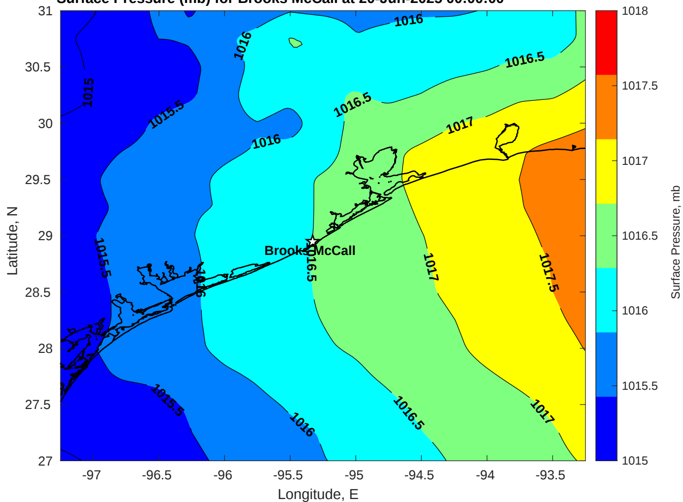
Surface Pressure (mb) for Brooks McCall at 20-Jun-2025 00:00:00
