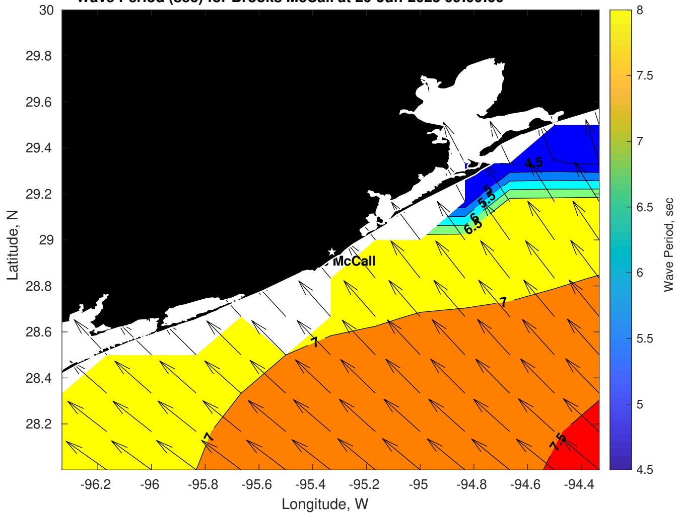
Wave Period (sec) for Brooks McCall at 20-Jun-2025 09:00:00
