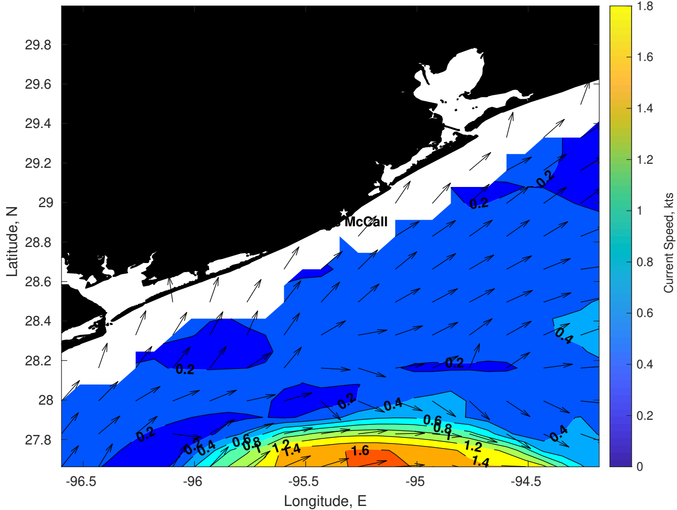
Surface Currents for Brooks McCall at 19-Jun-2025 00:00:00
