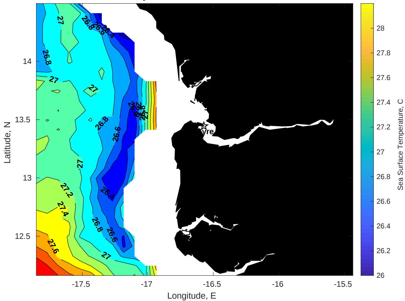
SST for Gyre at 19-Jun-2025 00:00:00
