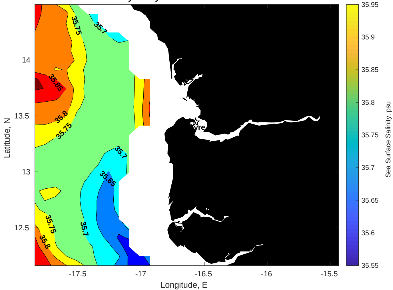
Surface Salinity for Gyre at 19-Jun-2025 00:00:00
