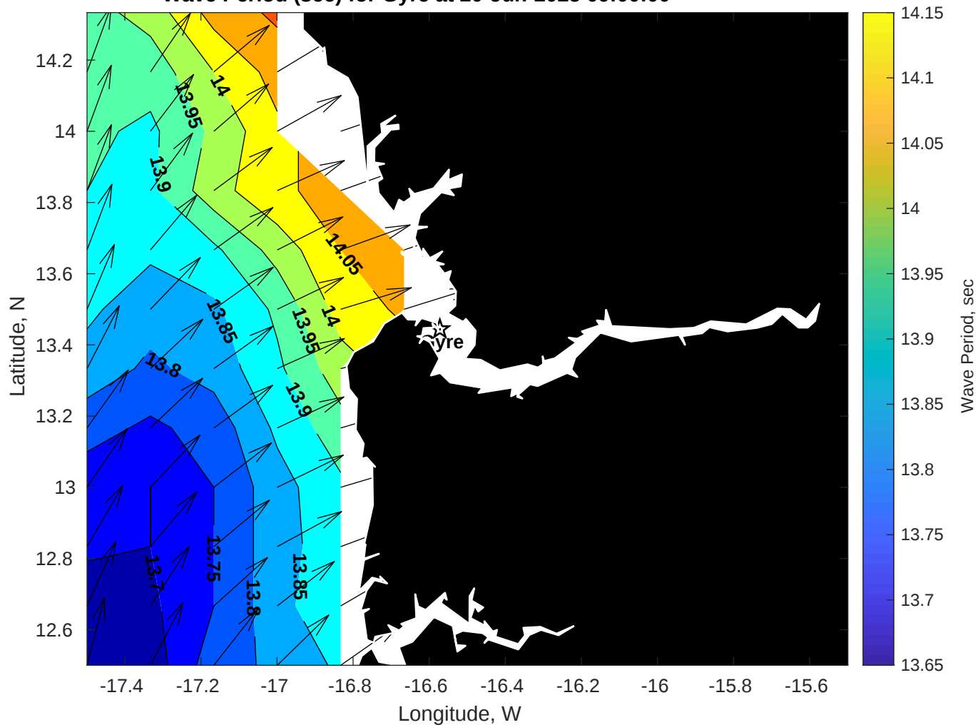
Wave Period (sec) for Gyre at 20-Jun-2025 09:00:00
