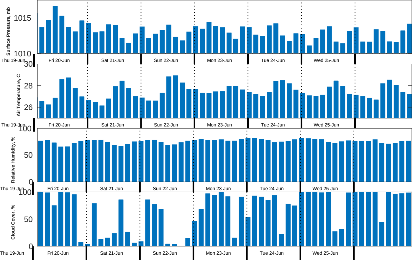
Met Forecast for Gyre from 19-Jun-2025 23:00:00 to 26-Jun-2025 23:00:00
