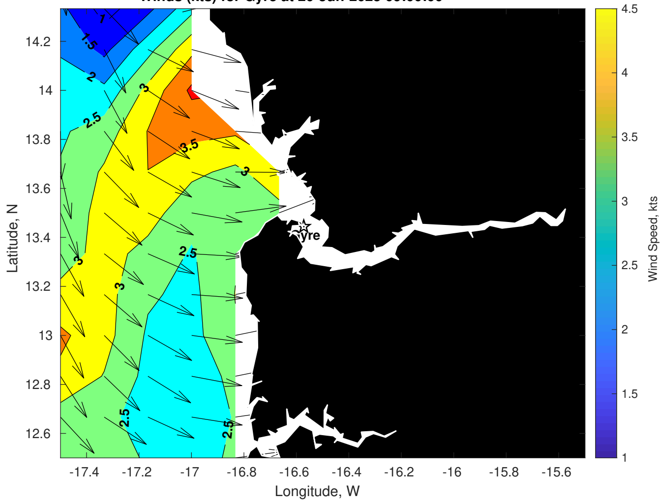
Winds (kts) for Gyre at 20-Jun-2025 09:00:00
