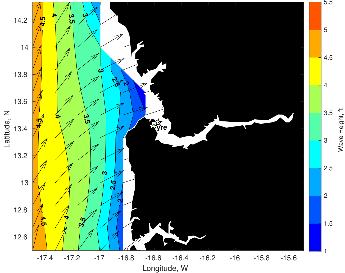
Wave Height (ft) for Gyre at 20-Jun-2025 09:00:00
