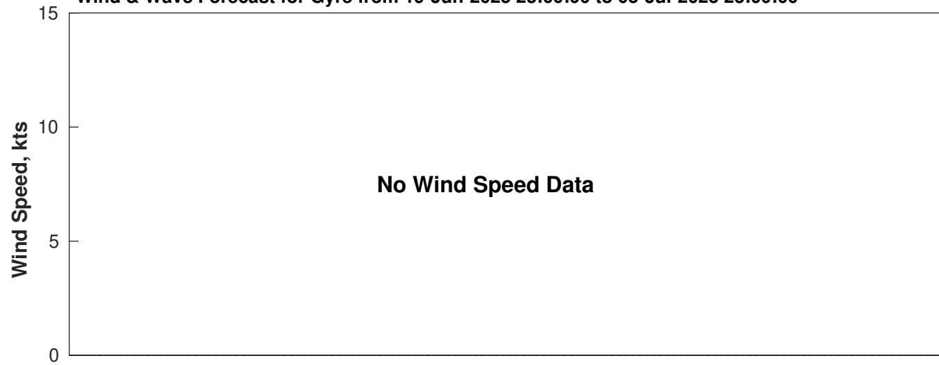
Wind & Wave Forecast for Gyre from 19-Jun-2025 23:00:00 to 05-Jul-2025 23:00:00
