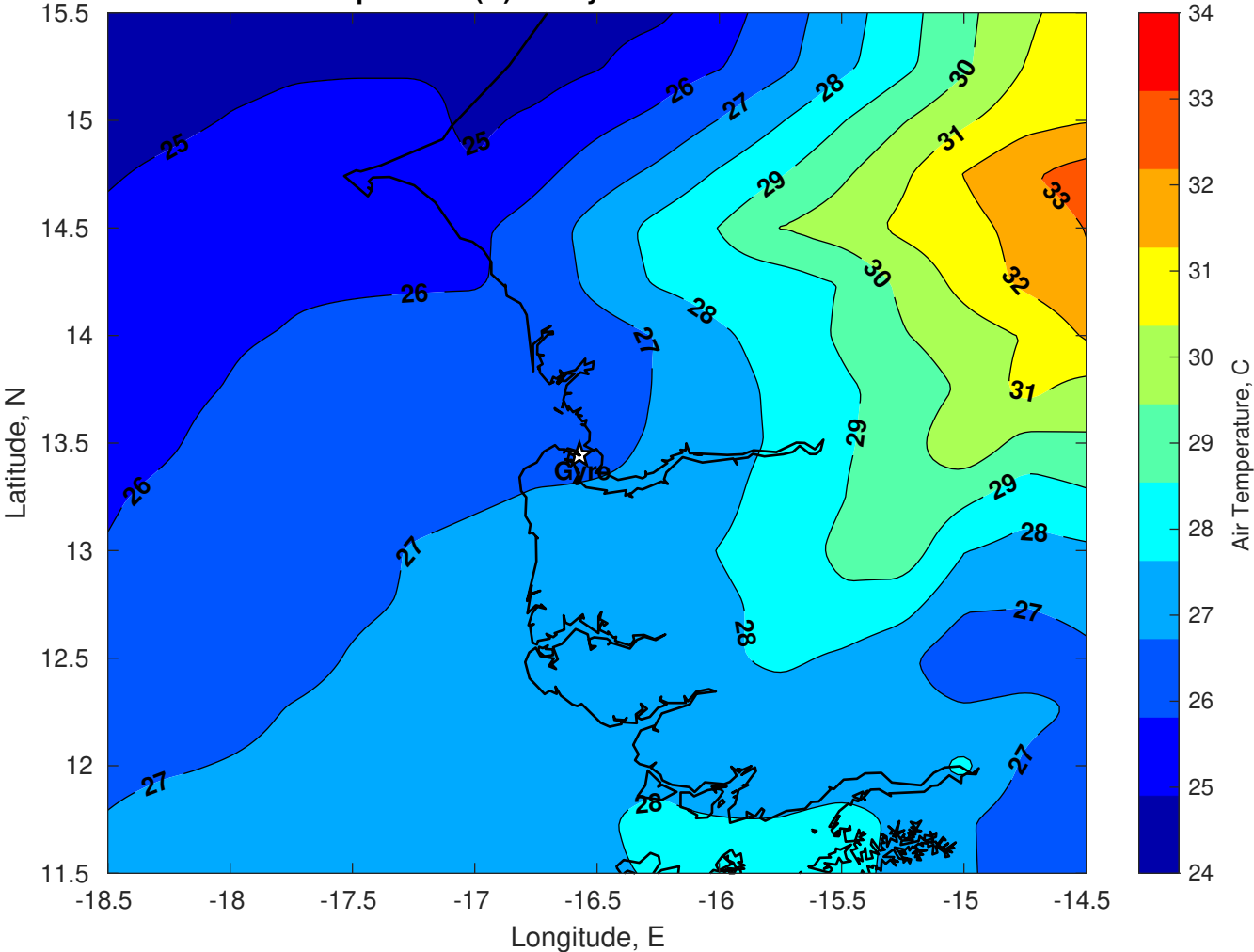
Air Temperature (C) for Gyre at 20-Jun-2025
