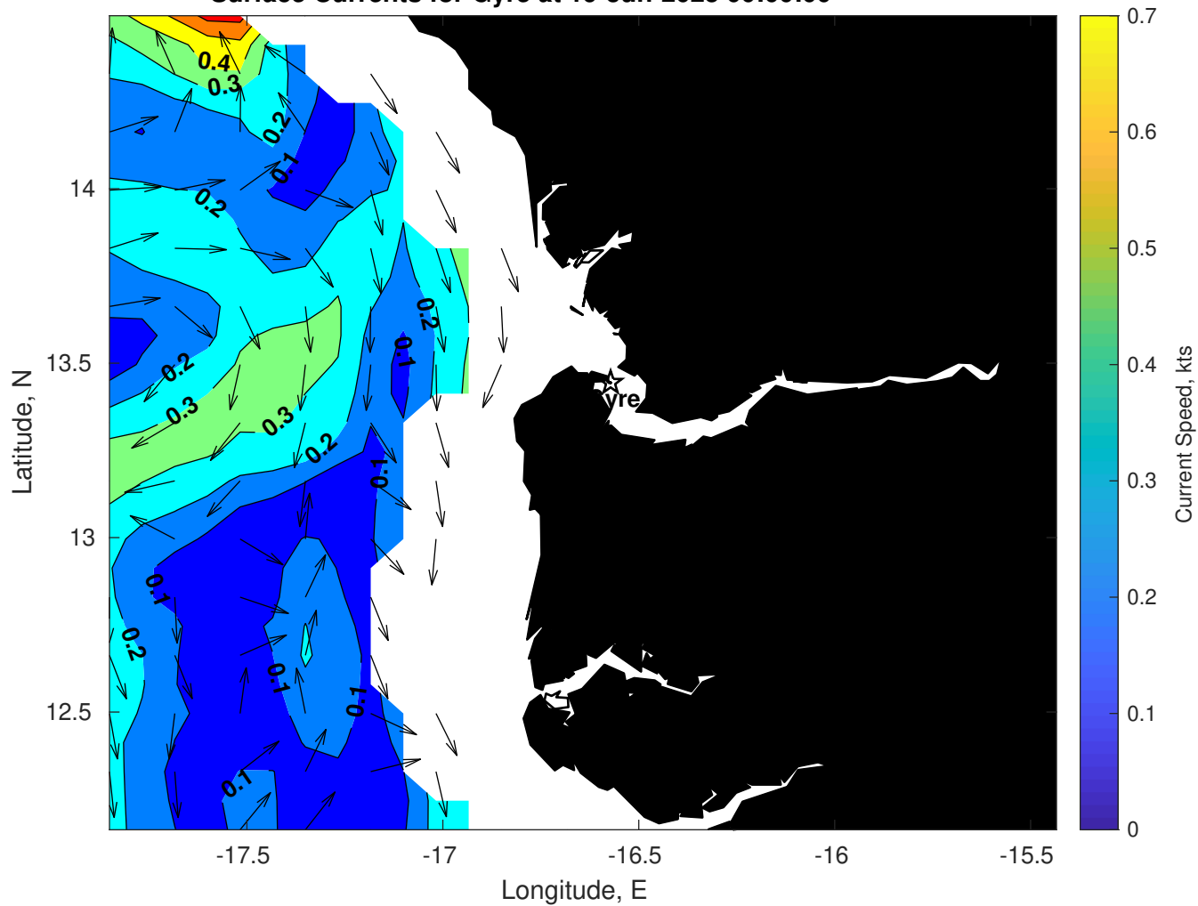
Surface Currents for Gyre at 19-Jun-2025 00:00:00
