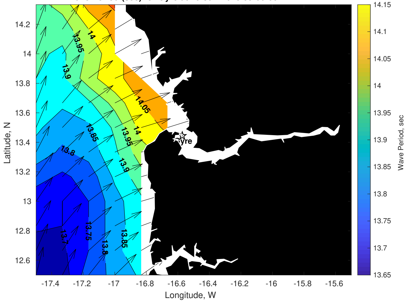
Wave Period (sec) for Gyre at 20-Jun-2025 09:00:00
