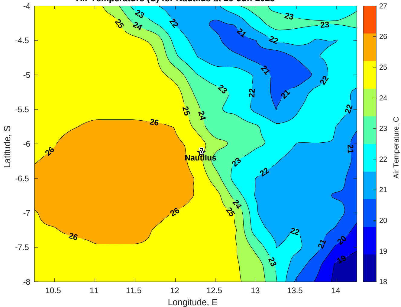
Air Temperature (C) for Nautilus at 20-Jun-2025
