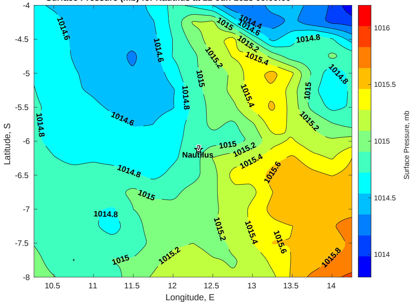
Surface Pressure (mb) for Nautilus at 22-Jun-2025 00:00:00
