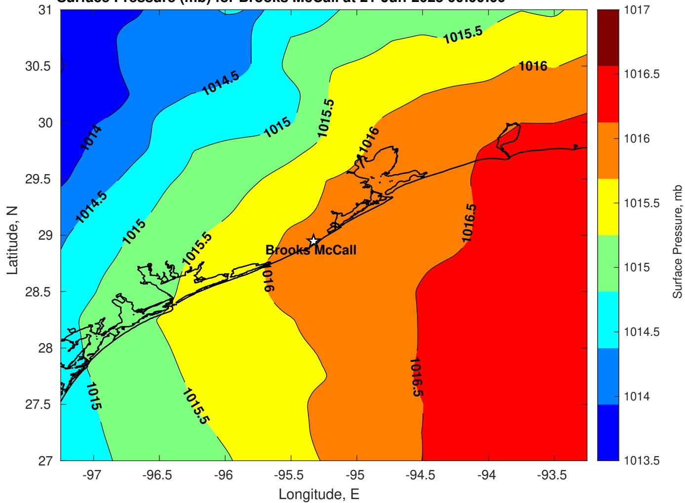
Surface Pressure (mb) for Brooks McCall at 21-Jun-2025 00:00:00
