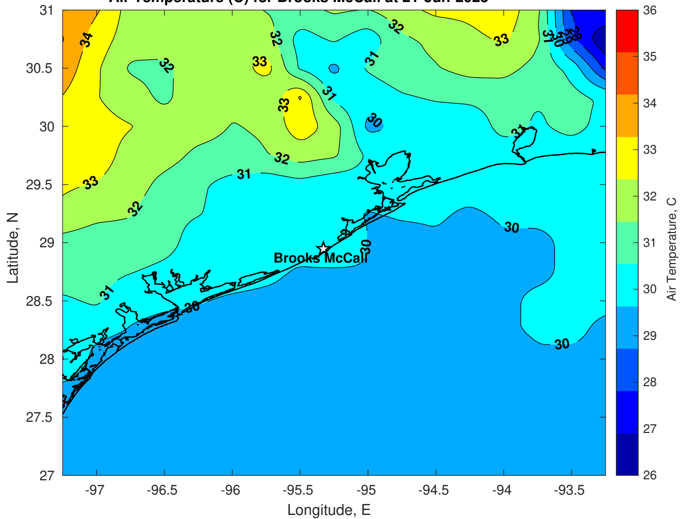
Air Temperature (C) for Brooks McCall at 21-Jun-2025
