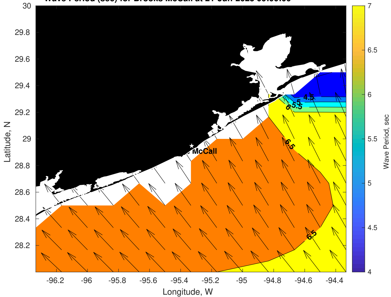
Wave Period (sec) for Brooks McCall at 21-Jun-2025 09:00:00
