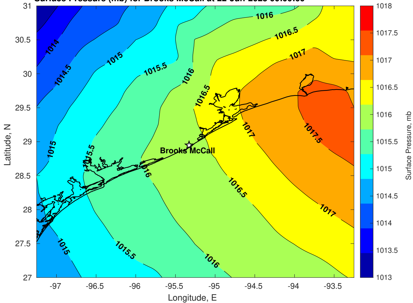
Surface Pressure (mb) for Brooks McCall at 22-Jun-2025 00:00:00
