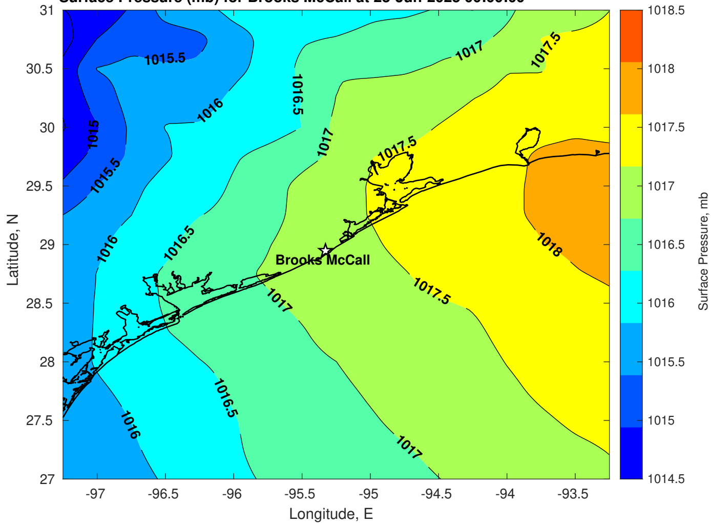
Surface Pressure (mb) for Brooks McCall at 23-Jun-2025 00:00:00
