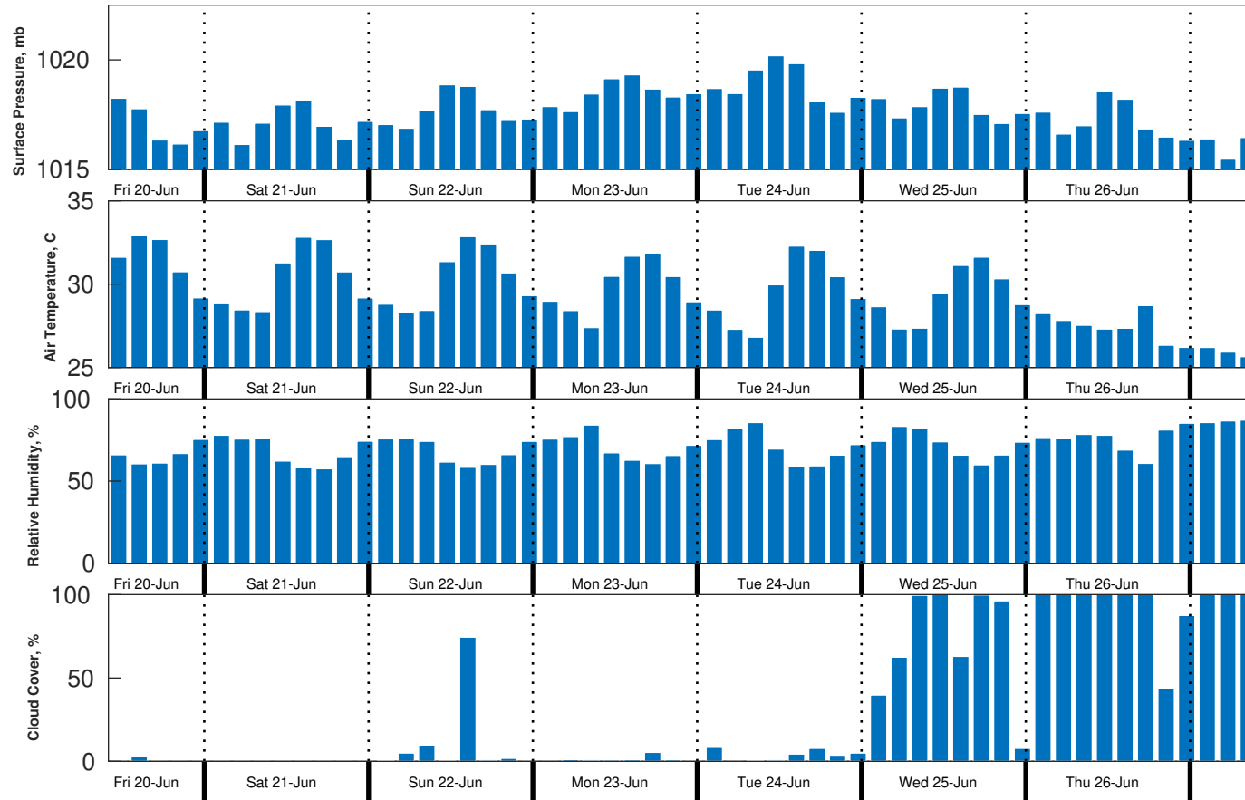
Met Forecast for Brooks McCall from 20-Jun-2025 12:00:00 to 27-Jun-2025 12:00:00
