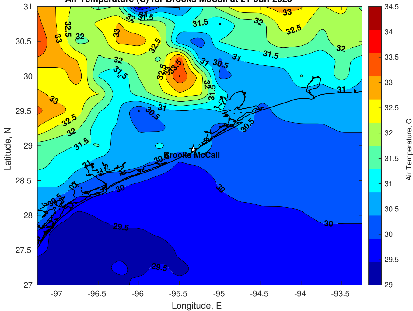
Air Temperature (C) for Brooks McCall at 21-Jun-2025
