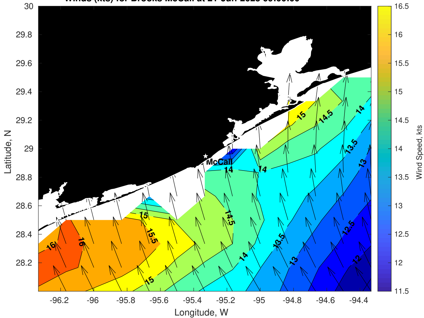
Winds (kts) for Brooks McCall at 21-Jun-2025 09:00:00
