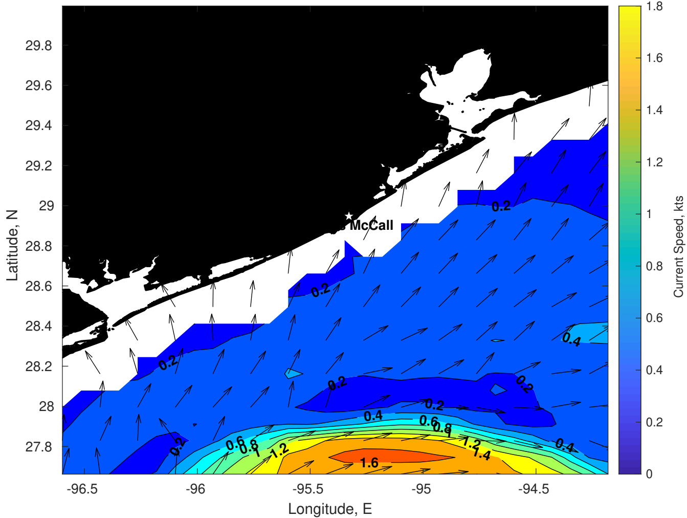
Surface Currents for Brooks McCall at 20-Jun-2025 00:00:00
