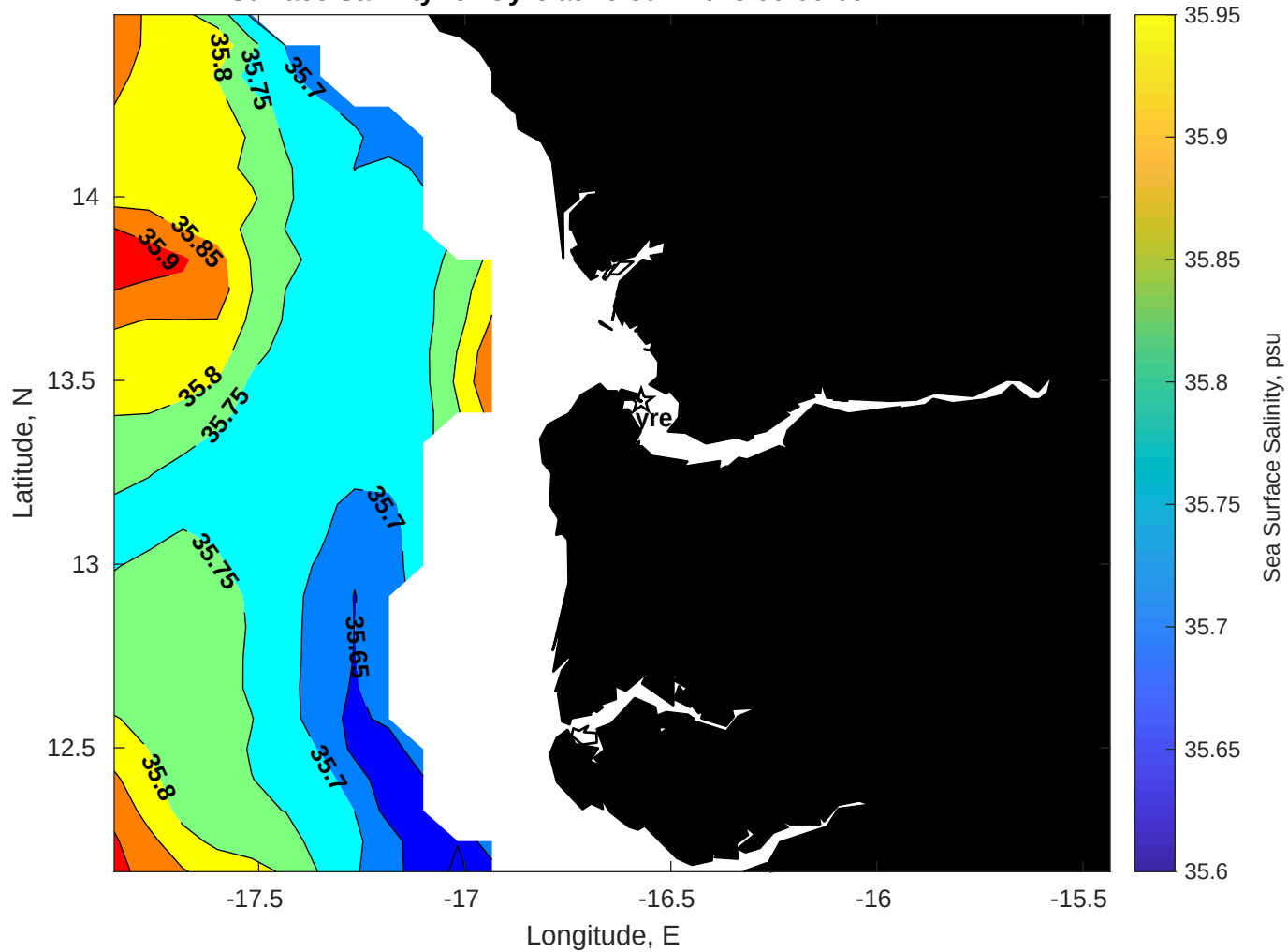
Surface Salinity for Gyre at 20-Jun-2025 00:00:00
