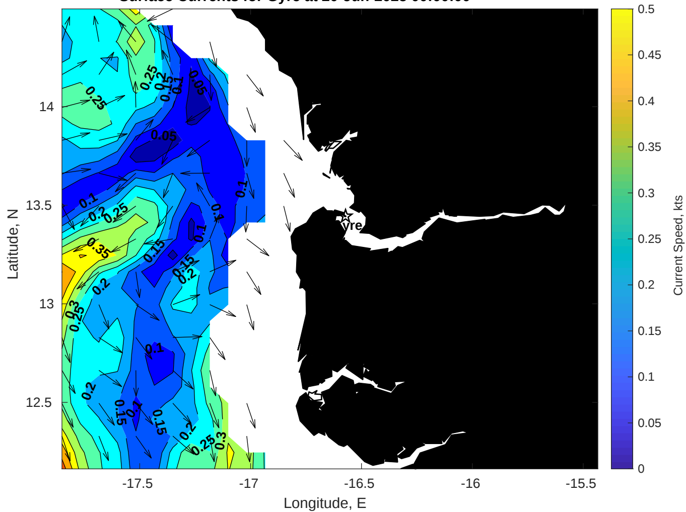
Surface Currents for Gyre at 20-Jun-2025 00:00:00
