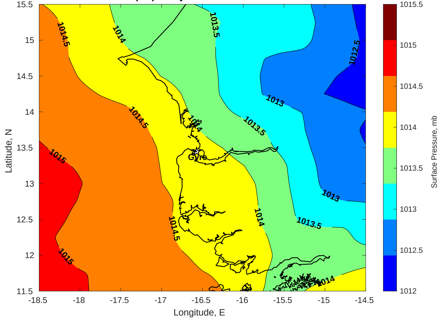
Surface Pressure (mb) for Gyre at 21-Jun-2025 00:00:00
