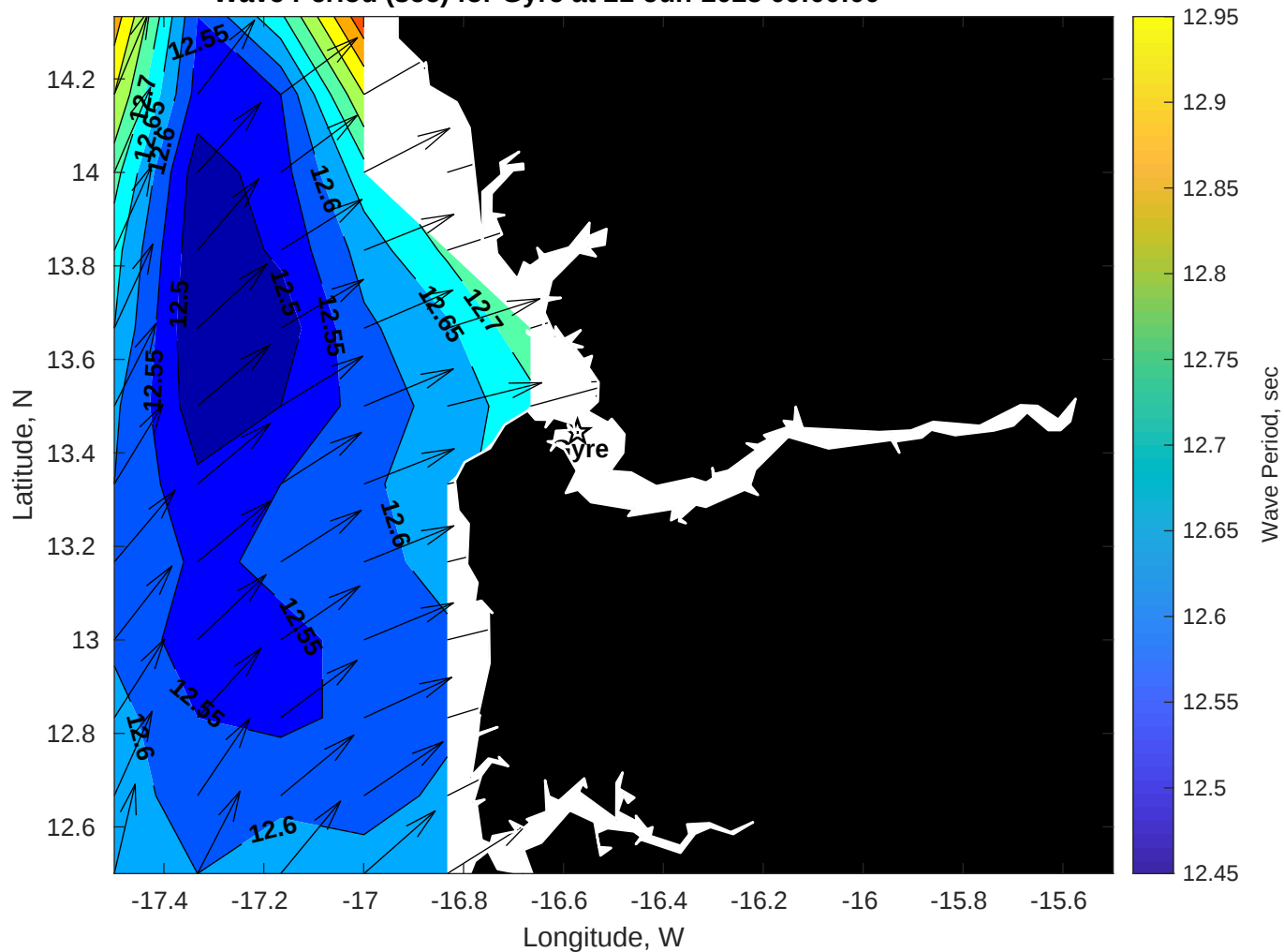
Wave Period (sec) for Gyre at 21-Jun-2025 09:00:00
