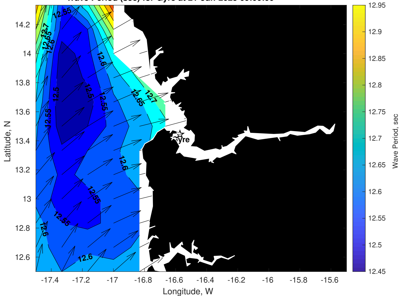
Wave Period (sec) for Gyre at 21-Jun-2025 09:00:00
