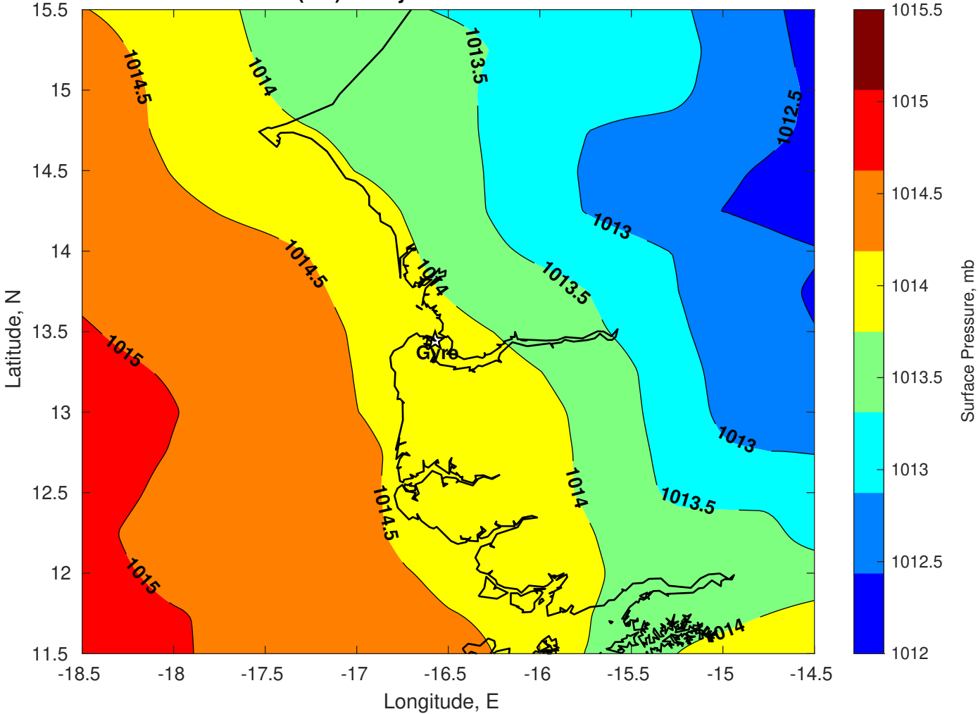
Surface Pressure (mb) for Gyre at 21-Jun-2025 00:00:00
