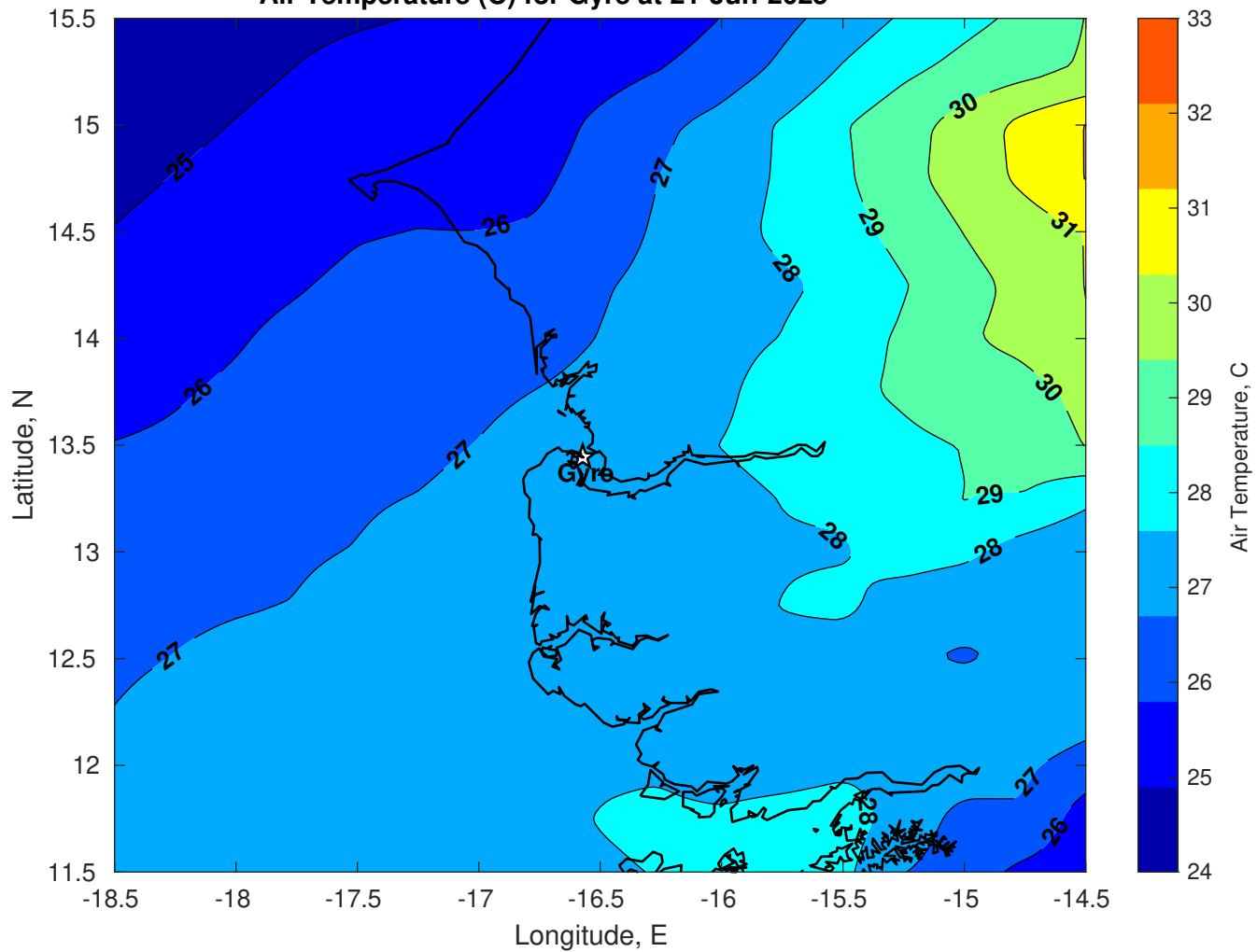
Air Temperature (C) for Gyre at 21-Jun-2025
