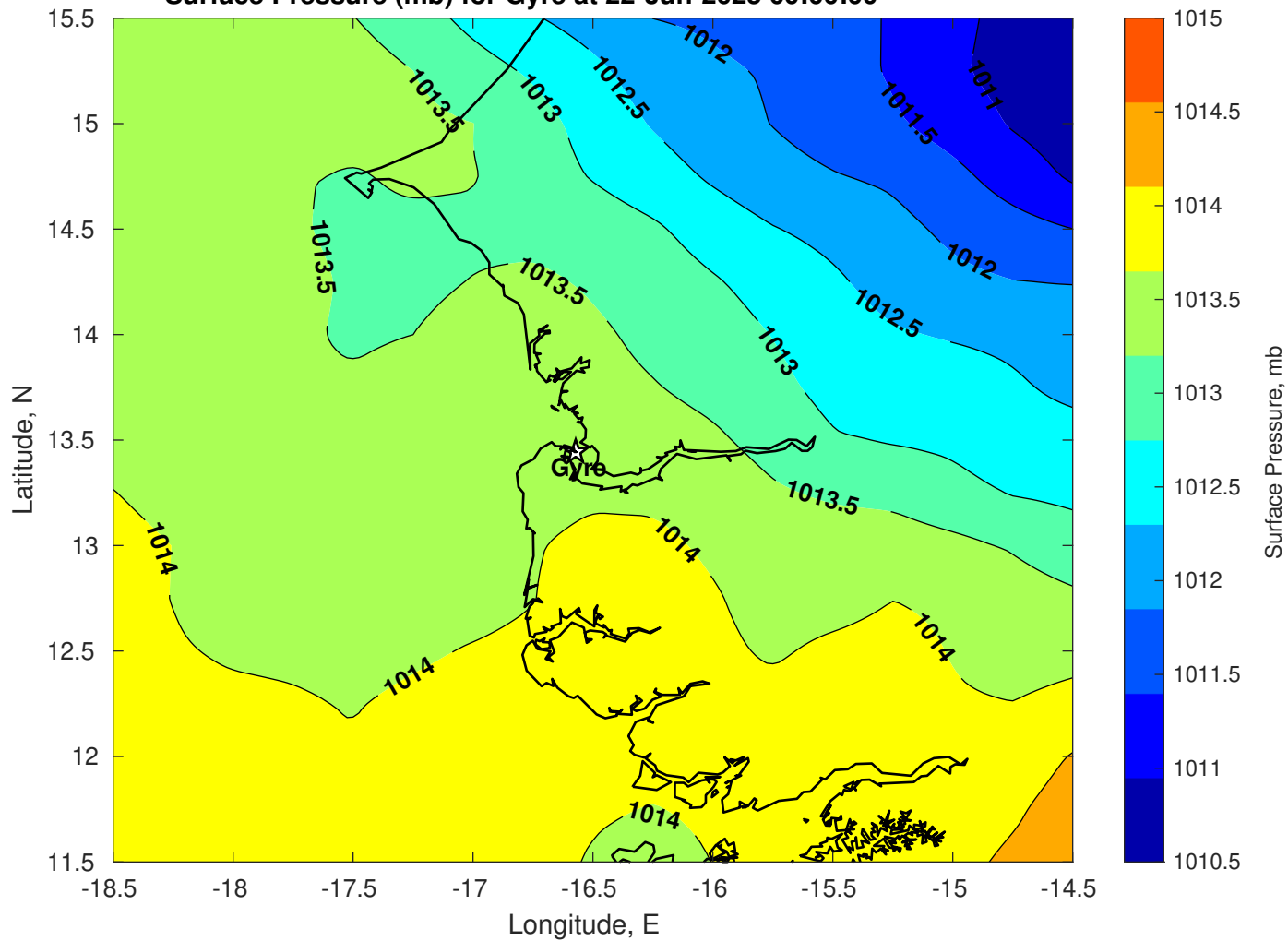
Surface Pressure (mb) for Gyre at 22-Jun-2025 00:00:00
