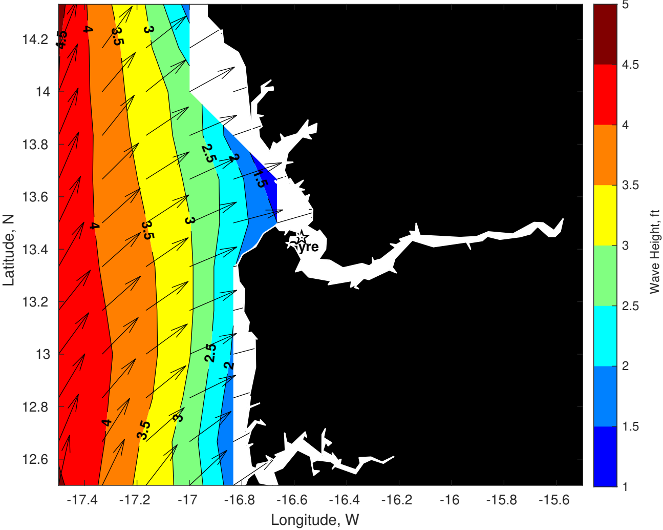
Wave Height (ft) for Gyre at 21-Jun-2025 09:00:00
