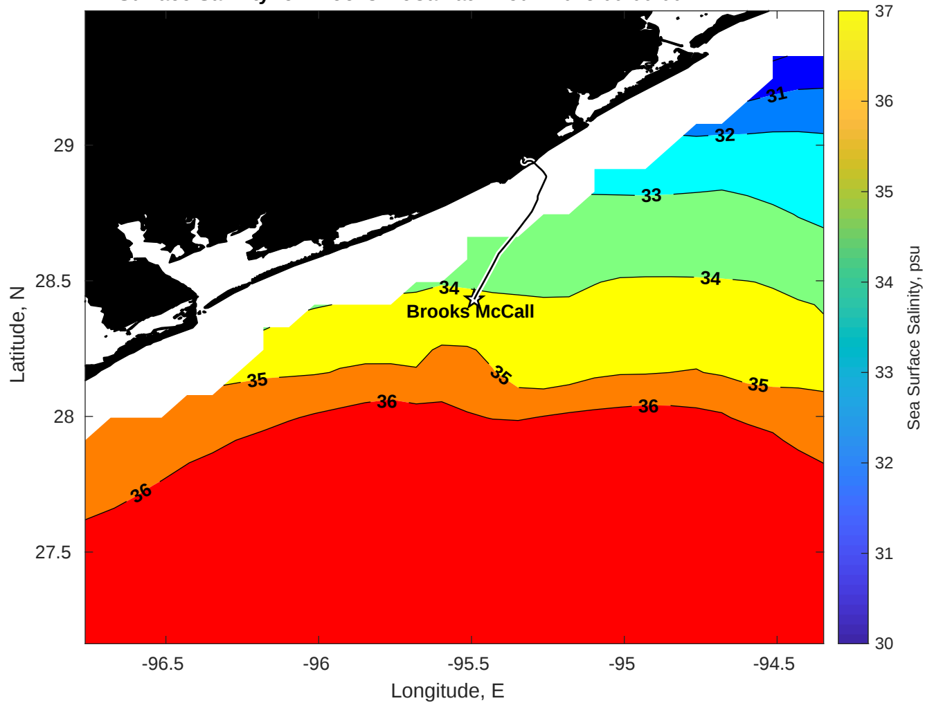
Surface Salinity for Brooks McCall at 21-Jun-2025 00:00:00
