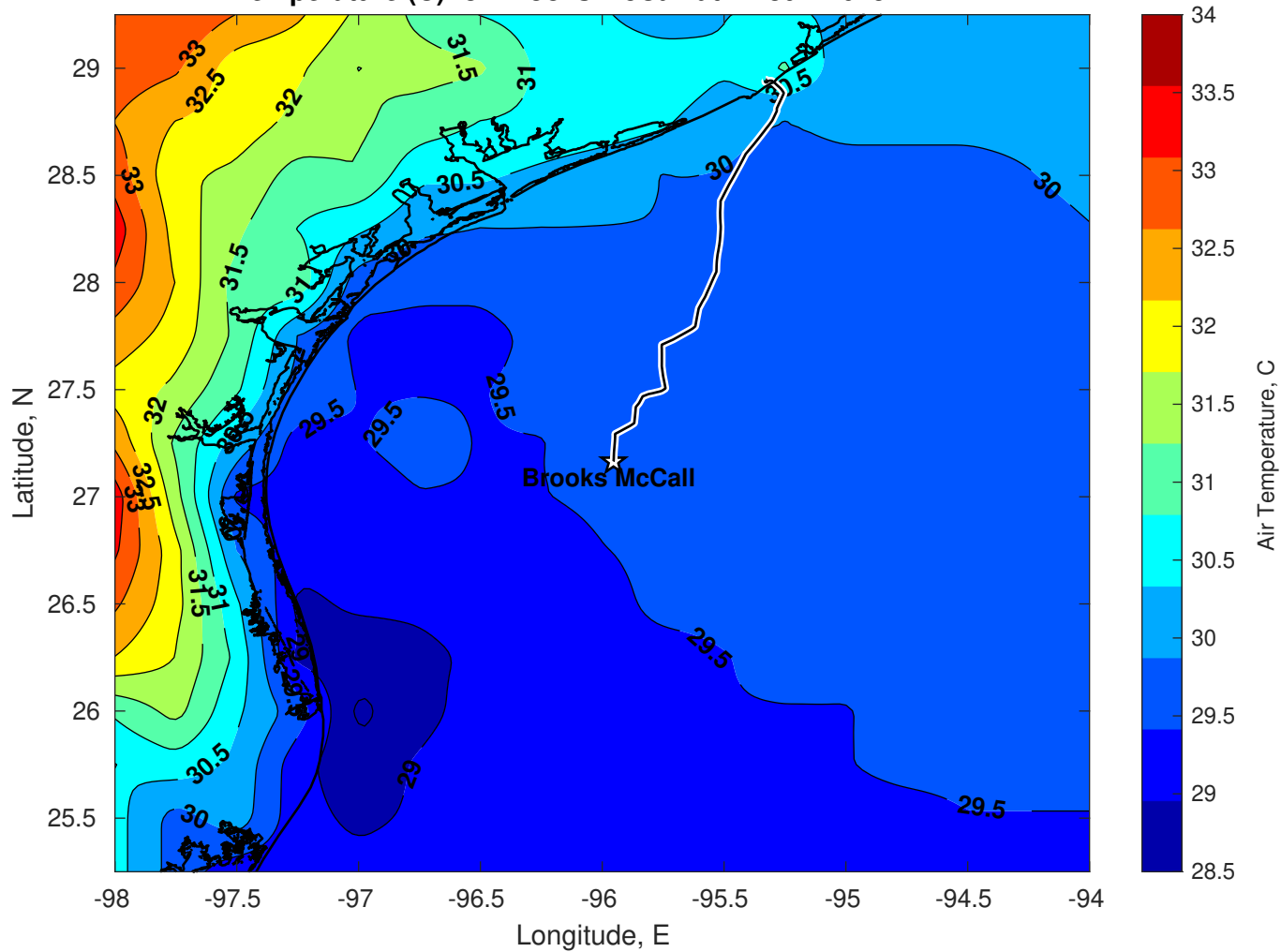
Air Temperature (C) for Brooks McCall at 22-Jun-2025
