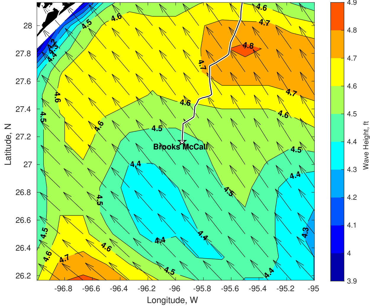
Wave Height (ft) for Brooks McCall at 22-Jun-2025 09:00:00
