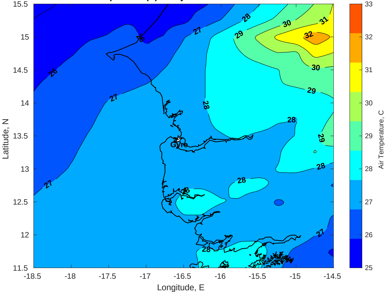
Air Temperature (C) for Gyre at 22-Jun-2025
