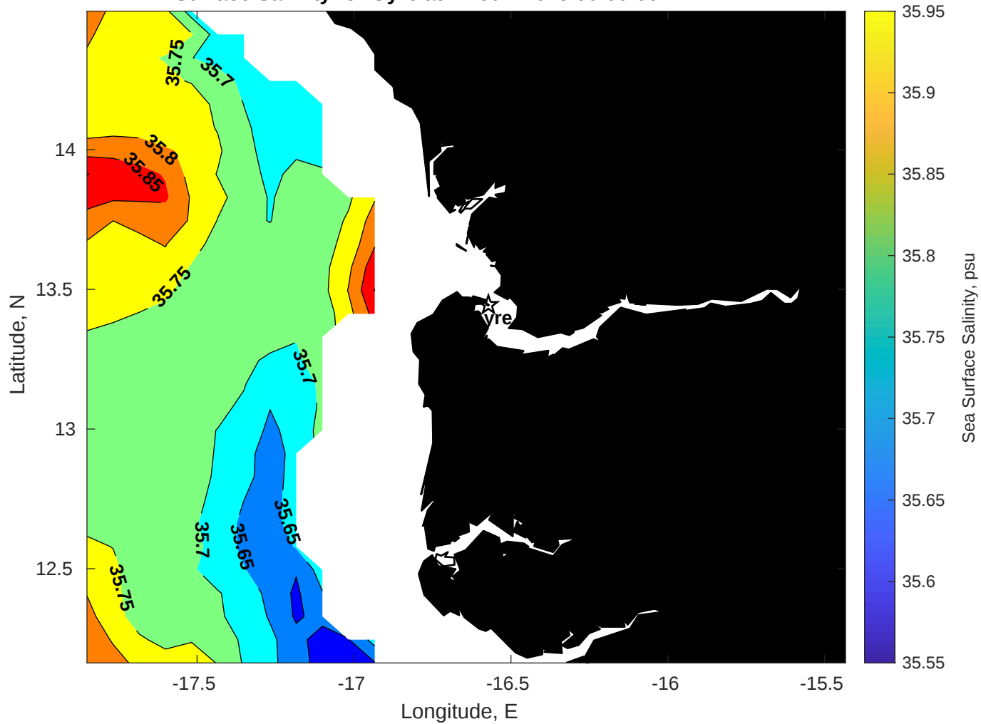
Surface Salinity for Gyre at 21-Jun-2025 00:00:00
