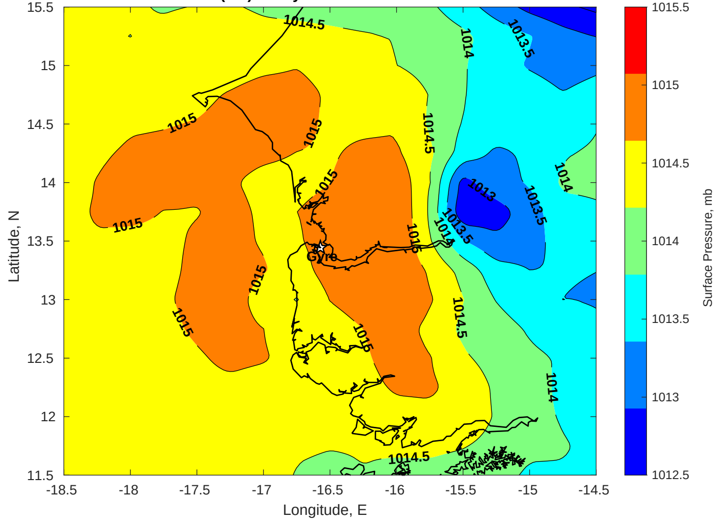
Surface Pressure (mb) for Gyre at 23-Jun-2025 00:00:00
