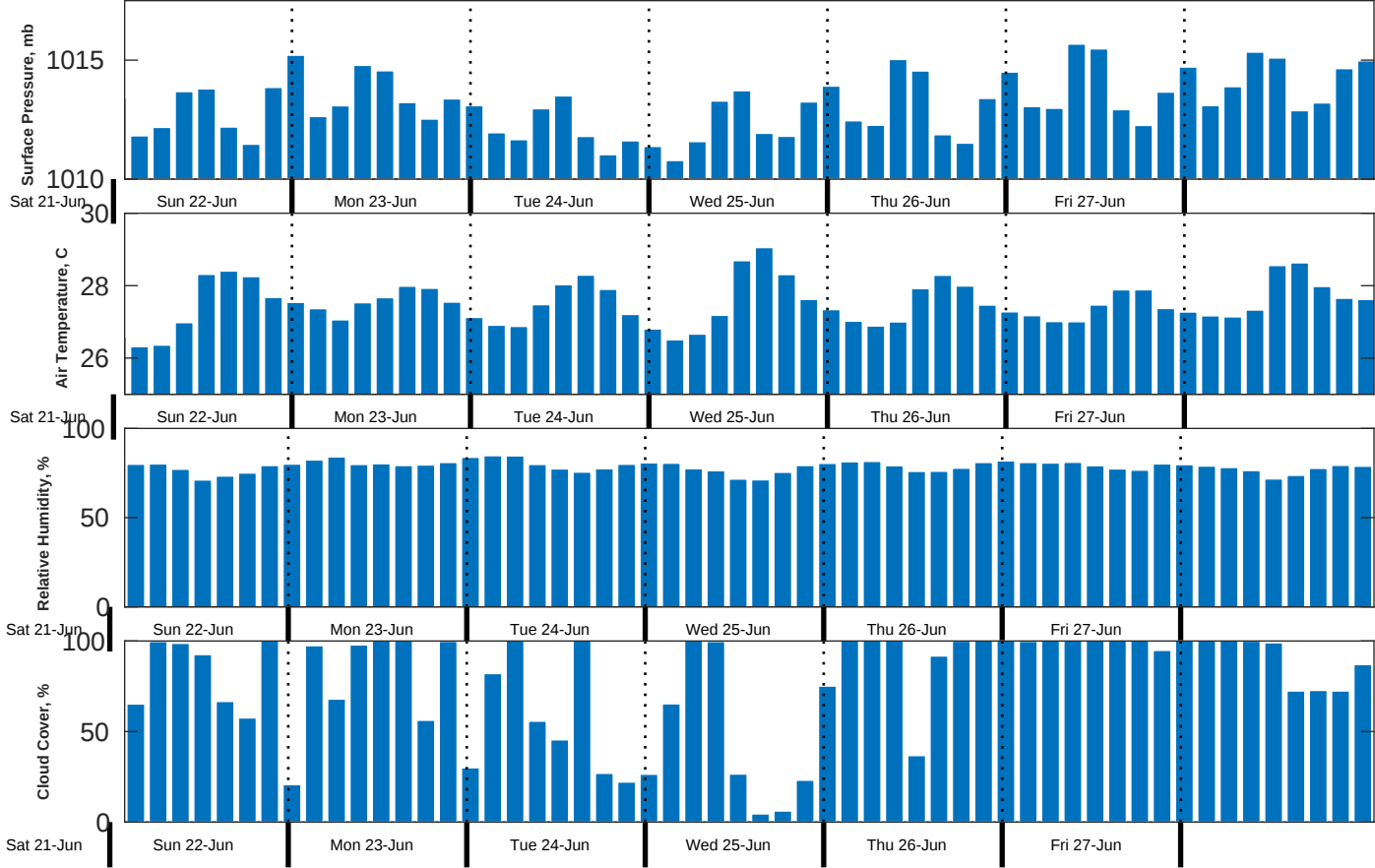
Met Forecast for Gyre from 21-Jun-2025 23:00:00 to 28-Jun-2025 23:00:00
