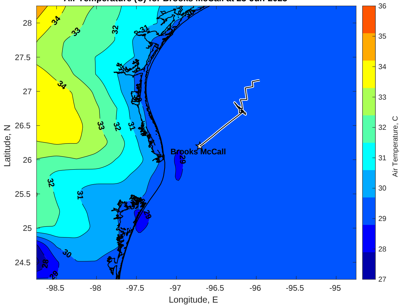
Air Temperature (C) for Brooks McCall at 23-Jun-2025
