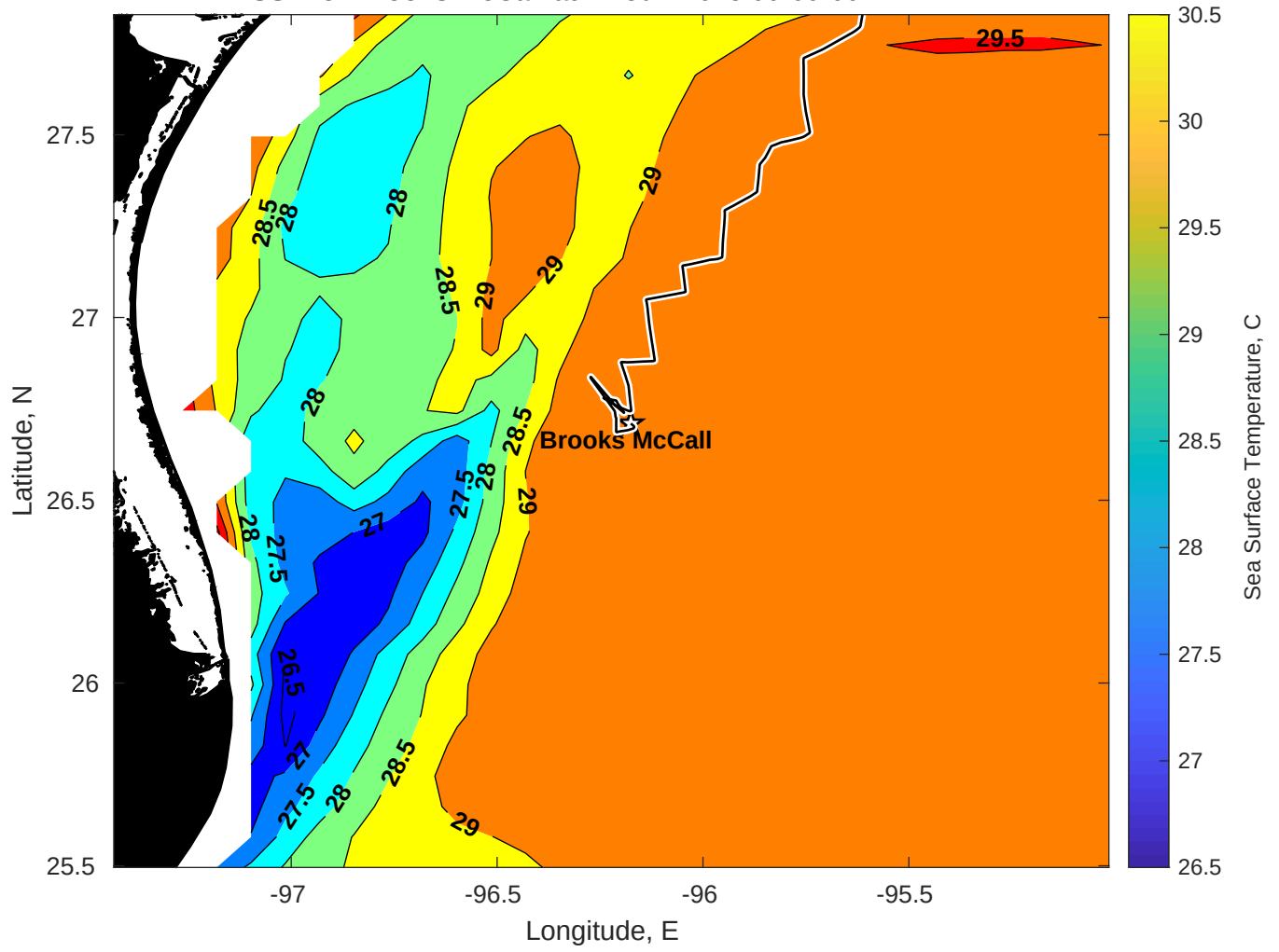
SST for Brooks McCall at 22-Jun-2025 00:00:00
