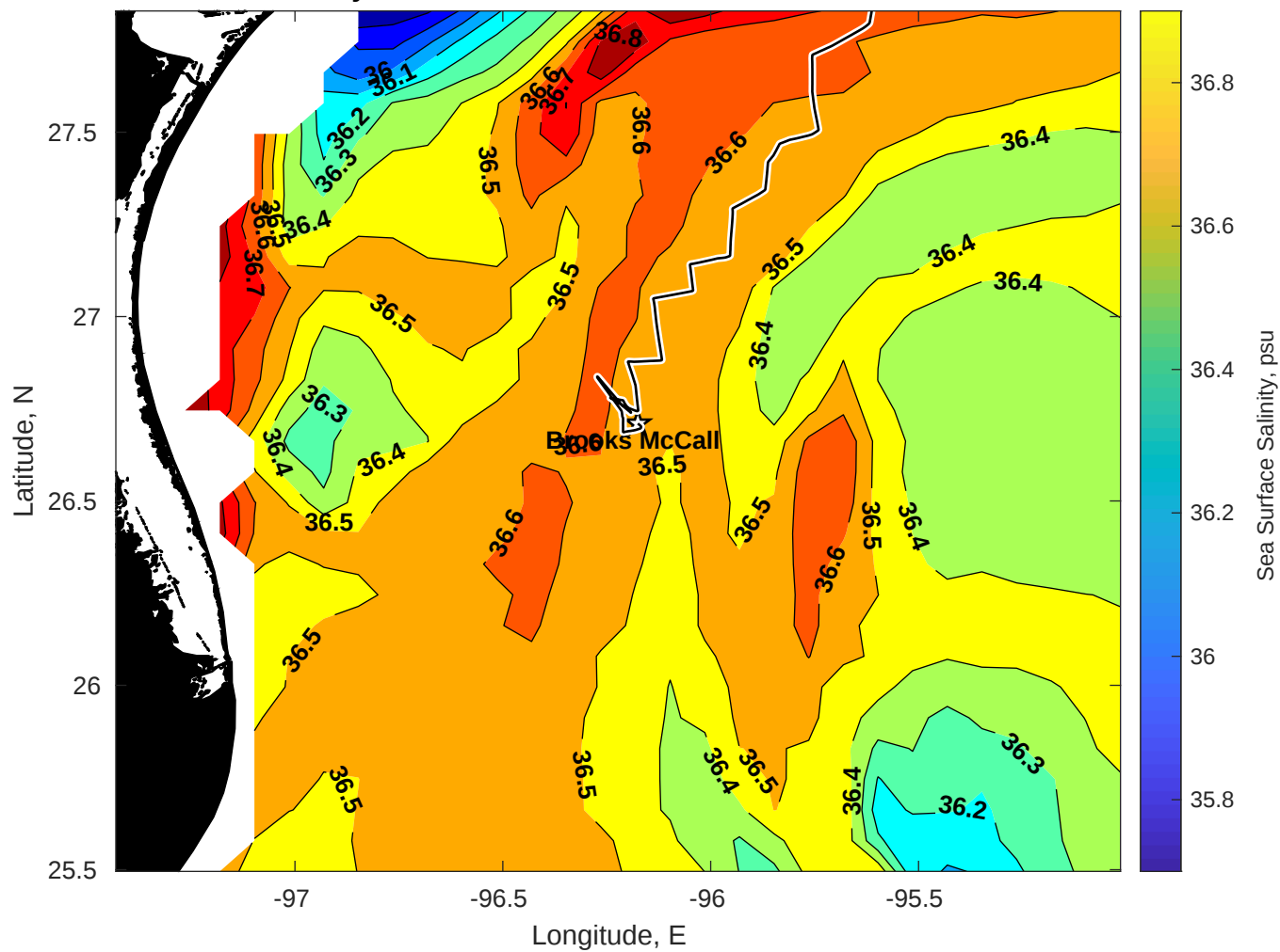
Surface Salinity for Brooks McCall at 22-Jun-2025 00:00:00
