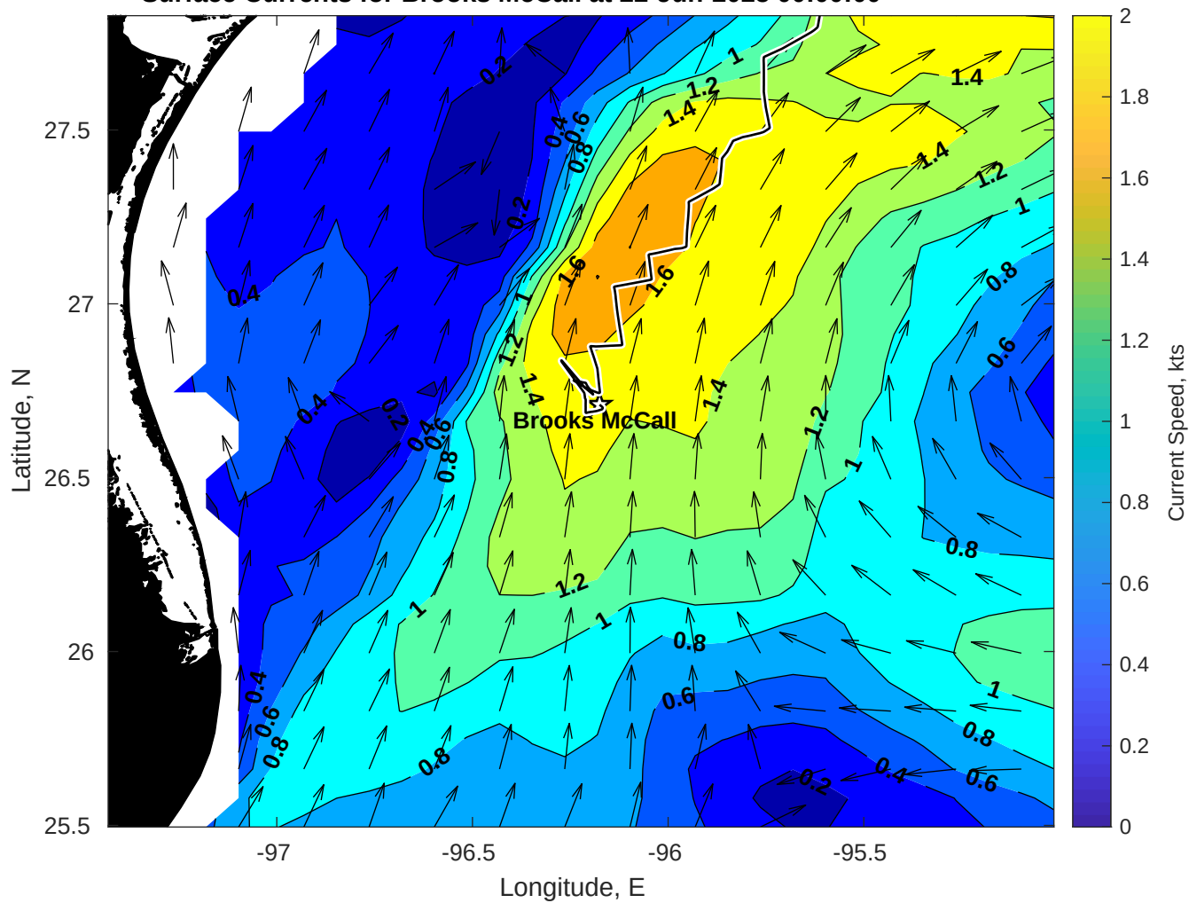
Surface Currents for Brooks McCall at 22-Jun-2025 00:00:00
