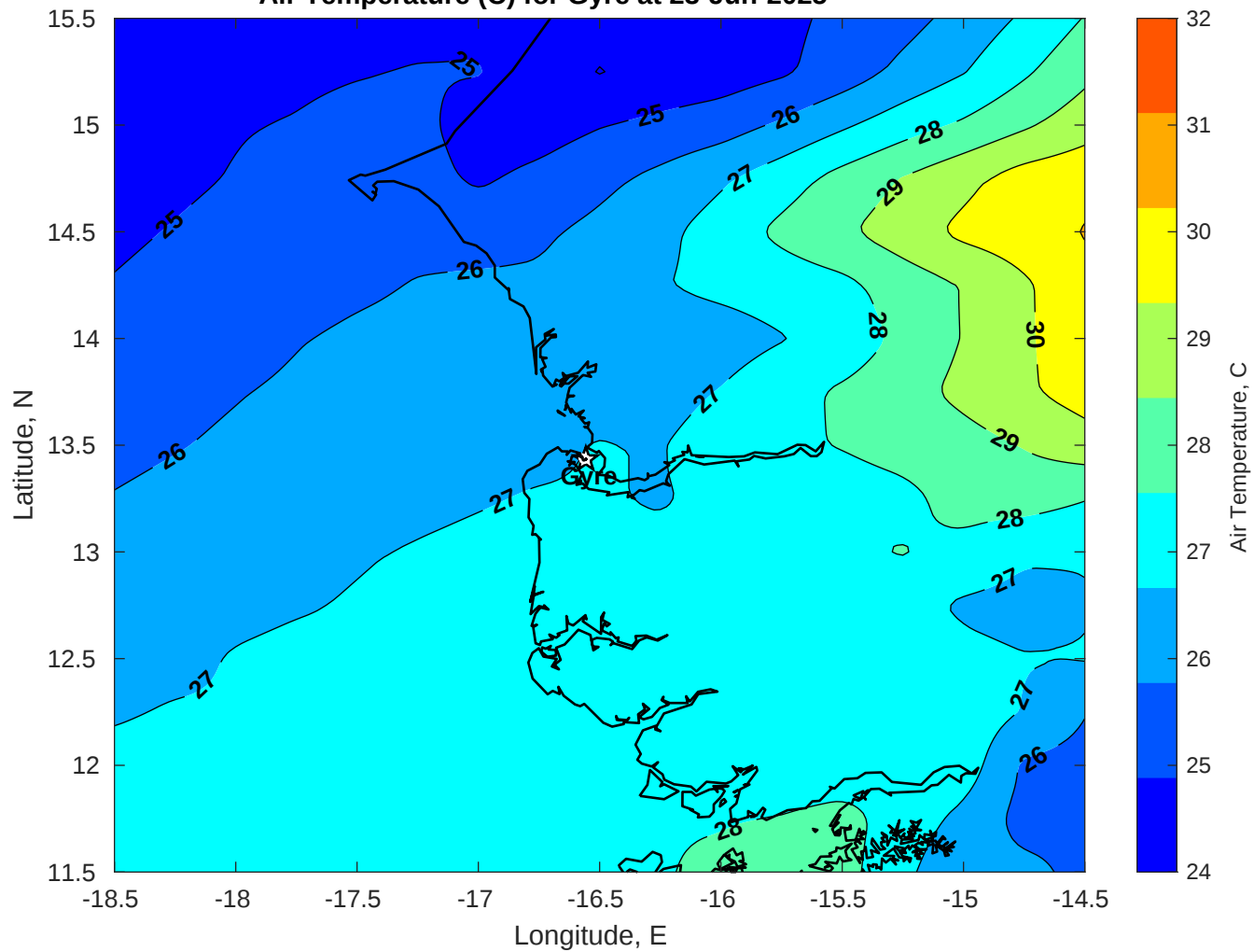
Air Temperature (C) for Gyre at 23-Jun-2025
