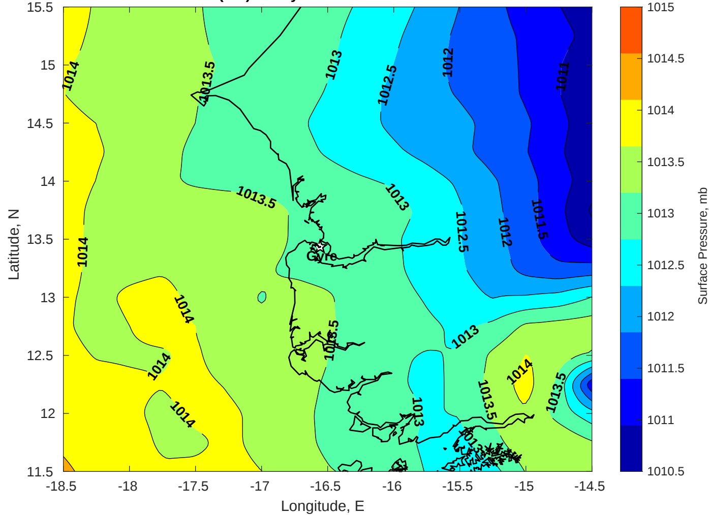
Surface Pressure (mb) for Gyre at 24-Jun-2025 00:00:00
