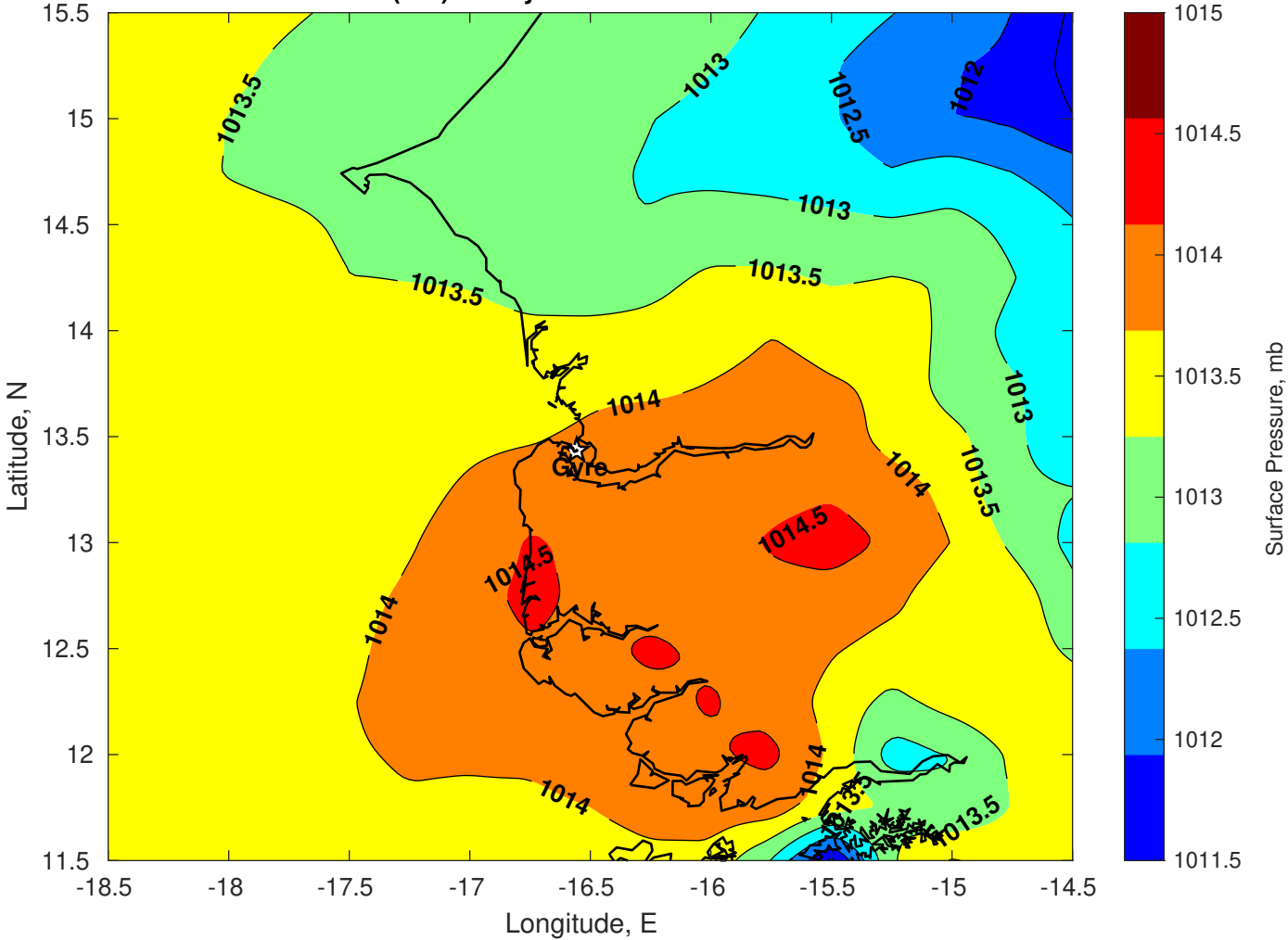
Surface Pressure (mb) for Gyre at 23-Jun-2025 00:00:00
