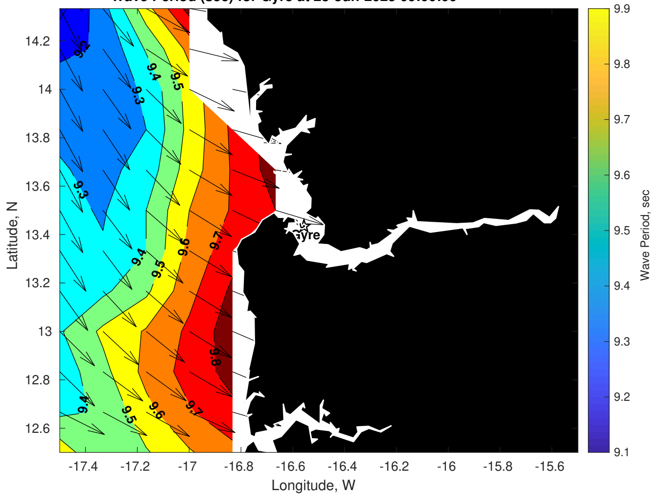
Wave Period (sec) for Gyre at 23-Jun-2025 09:00:00
