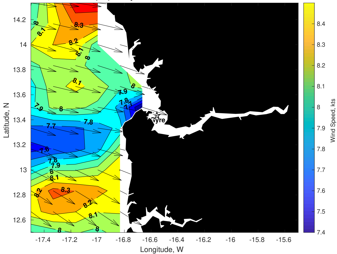
Winds (kts) for Gyre at 23-Jun-2025 09:00:00
