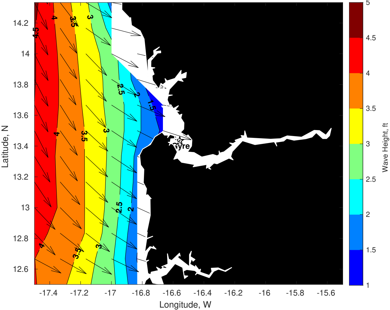
Wave Height (ft) for Gyre at 23-Jun-2025 09:00:00
