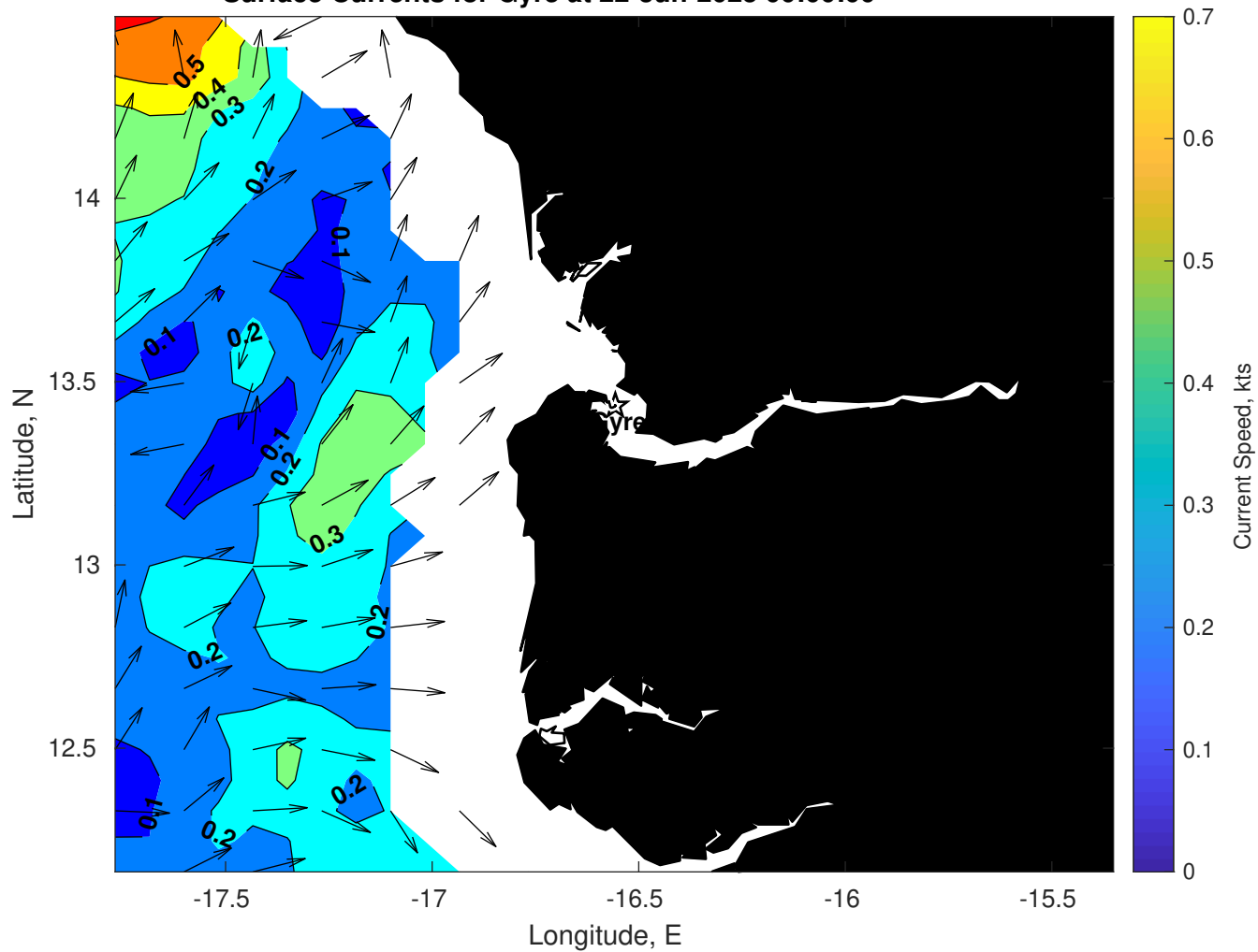
Surface Currents for Gyre at 22-Jun-2025 00:00:00
