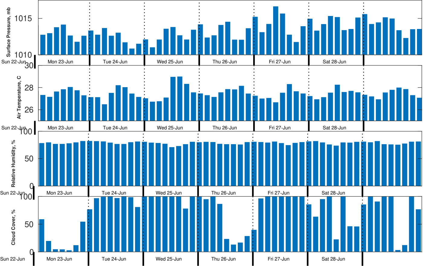
Met Forecast for Gyre from 22-Jun-2025 23:00:00 to 29-Jun-2025 23:00:00
