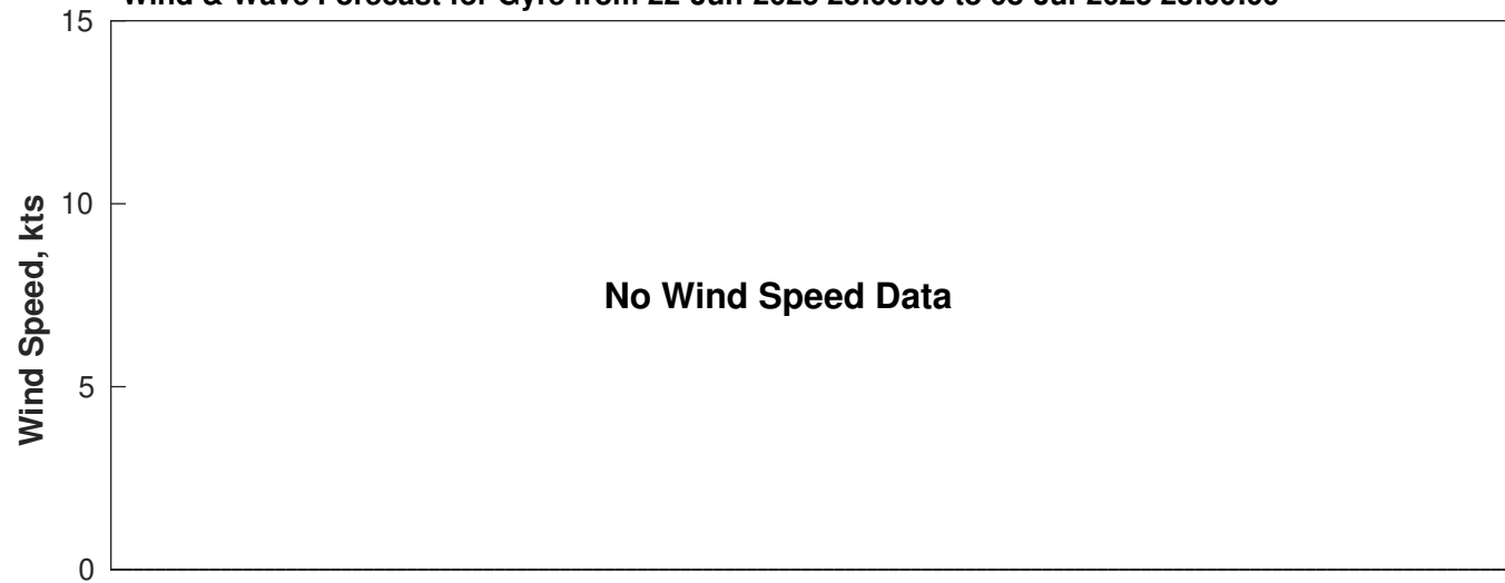
Wind & Wave Forecast for Gyre from 22-Jun-2025 23:00:00 to 08-Jul-2025 23:00:00
