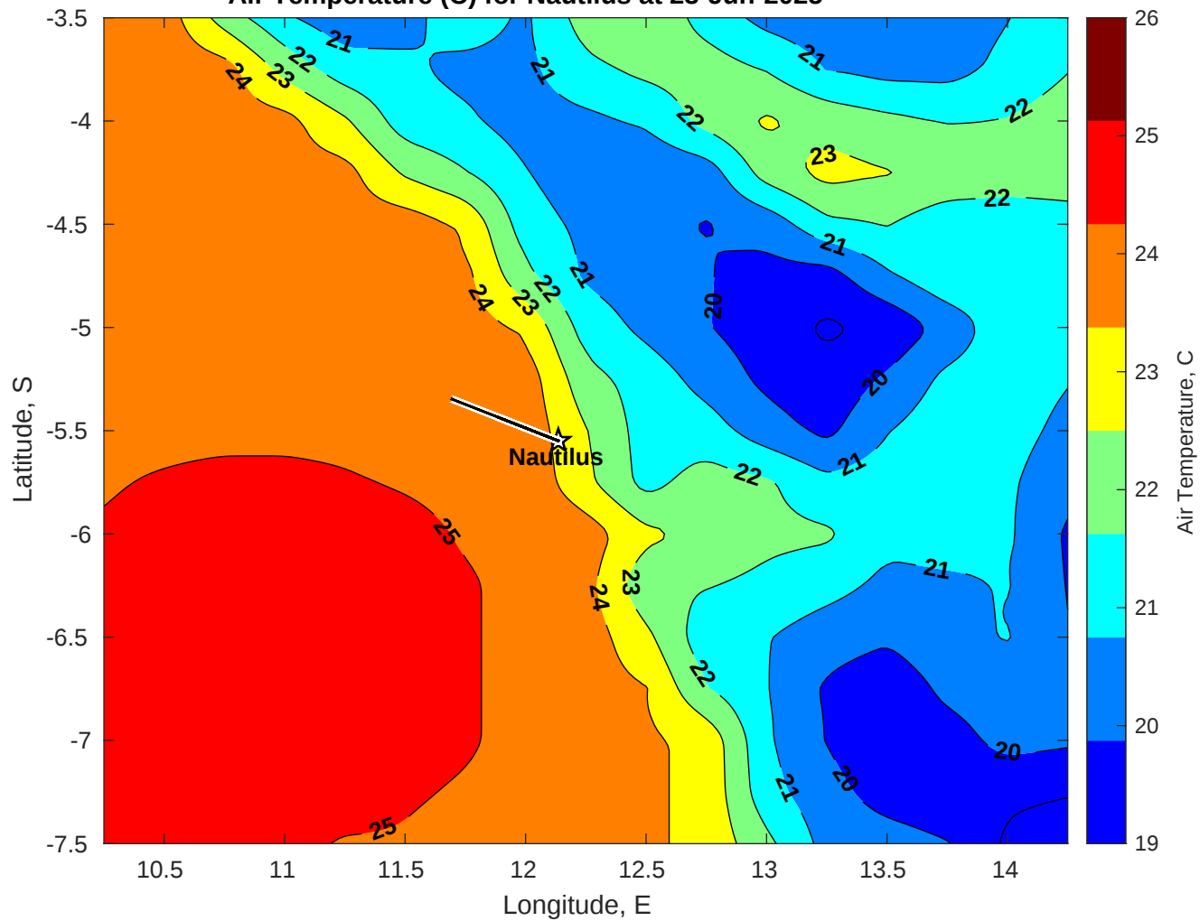
Air Temperature (C) for Nautilus at 23-Jun-2025
