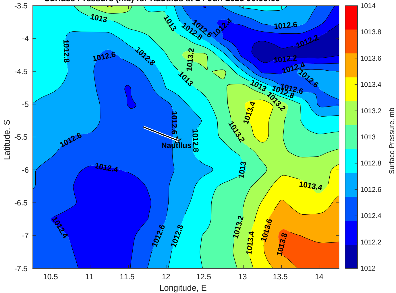
Surface Pressure (mb) for Nautilus at 24-Jun-2025 00:00:00
